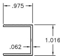
9 SASH STOP
