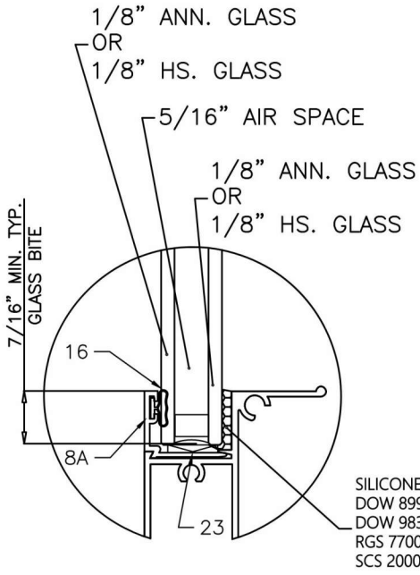
9/16" INSUL. GLASS
