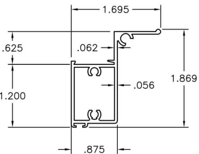
6 VENT BOTTOM RAIL
