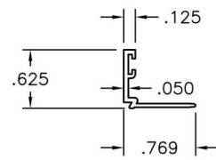
8A GLAZING BEAD (9/16" INSUL. GLASS)
