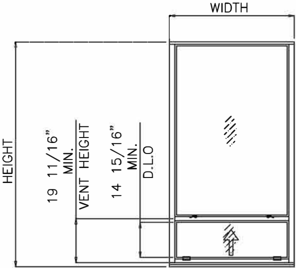
UNEQUAL LITES (ORIEL TYPE)
