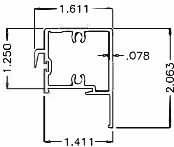
⑤ VENT TOP RAIL
