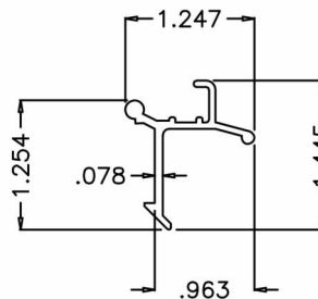
⑪ SPRING LOADED LATCH
