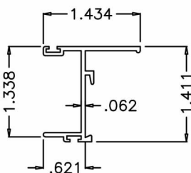
⑦ VENT SIDE RAIL
