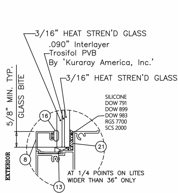
GLASS TYPE 'G1'
