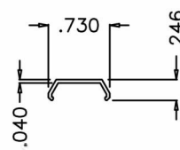
⑩ SCREW COVER
