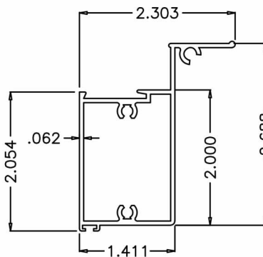
⑥ VENT BOTTOM RAIL
