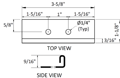
FLOATING BASE (PART No. 05082I)
