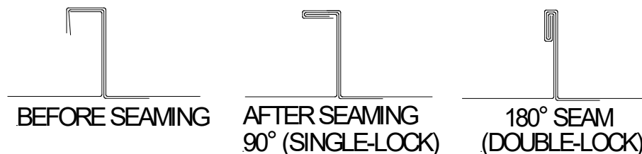
Panel Seaming Profiles
