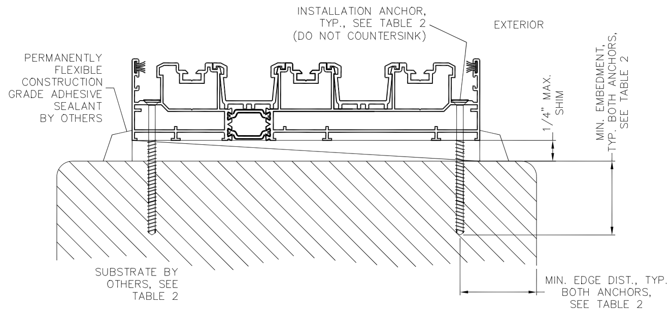
TYPICAL INSTALLATION AT TRIPLE FRAME HEAD, SILL, AND JAMB
