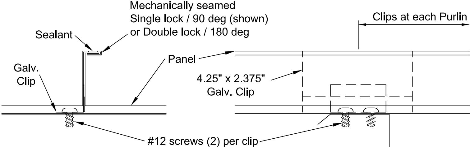
Clip Details
