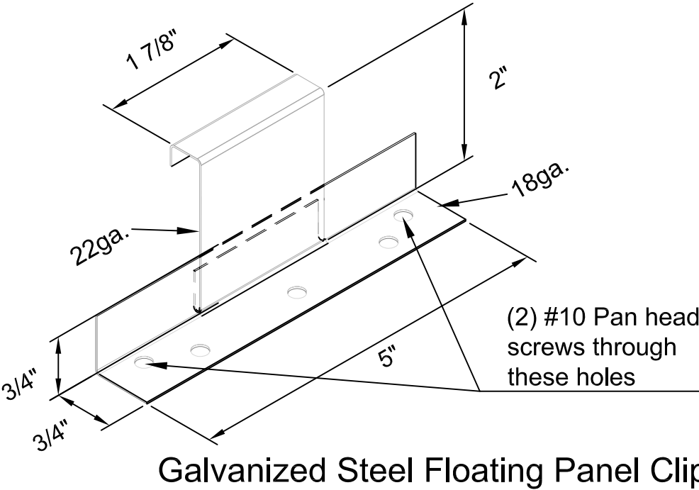
Clip Details
