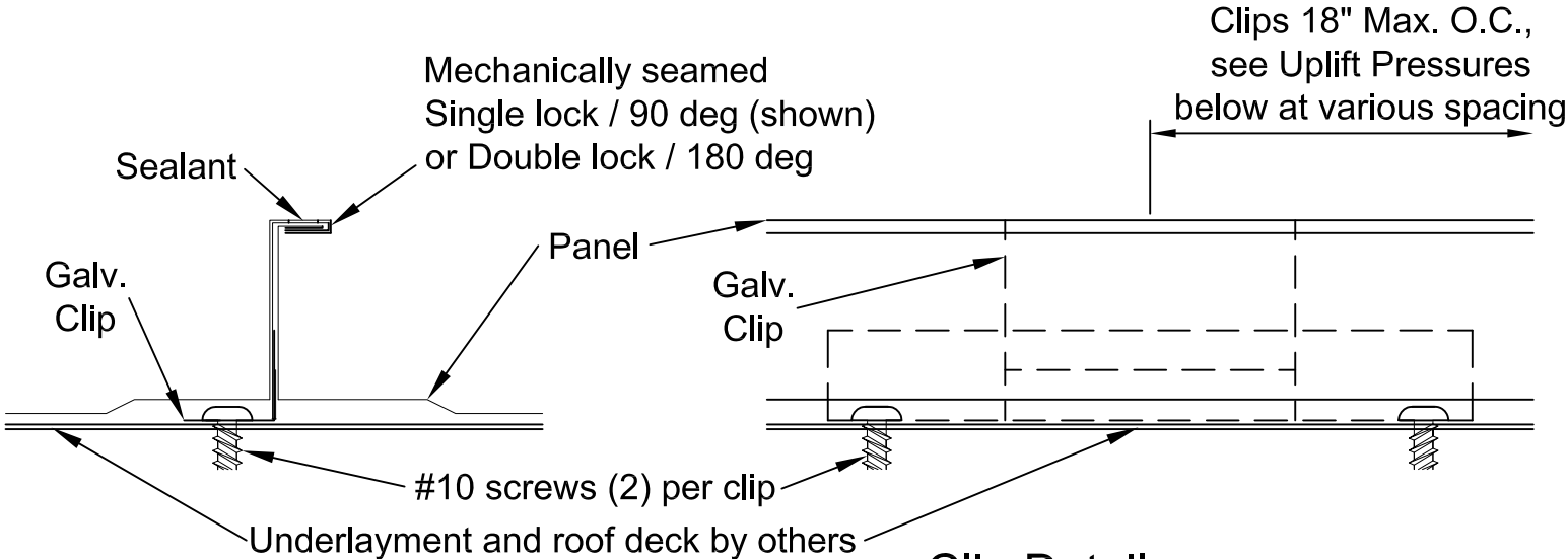
Clip Details
