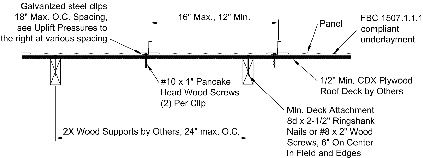
Typical Panel Installation
