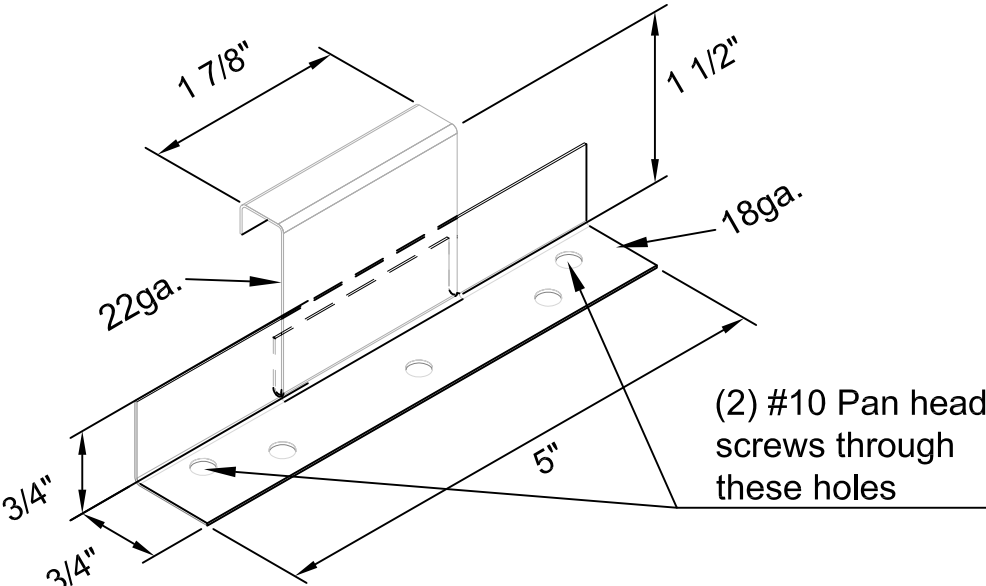
Galvanized Steel Floating Panle Clip
