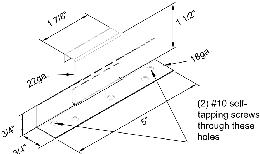
Galvanized Steel Floating Panel Clip
