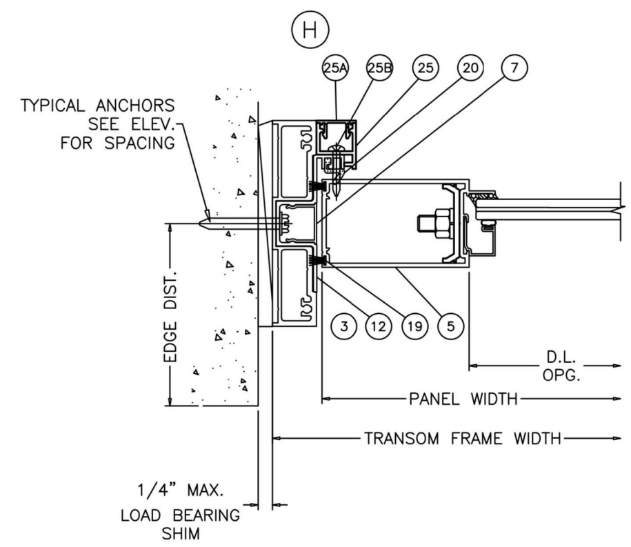
SIDELITE DETAILS
