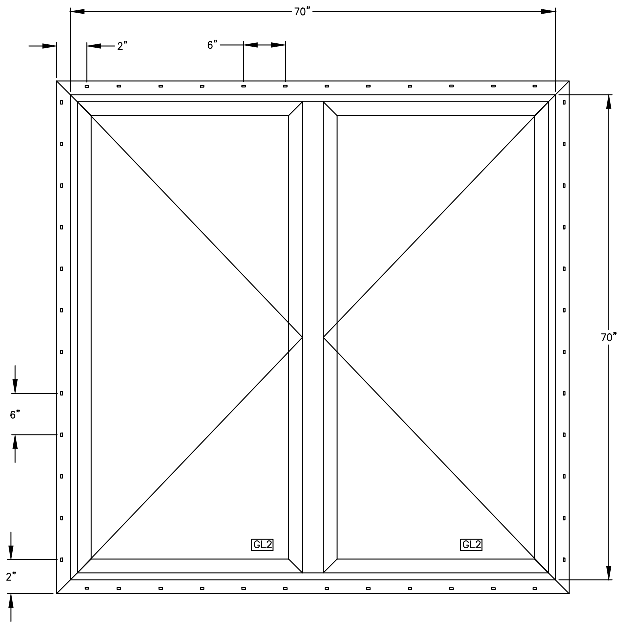
ASPECT/ENDURE T-MULL CASEMENT WINDOW (NON-IMPACT) MAXIMUM SIZE: 70" X 70" DESIGN PRESSURE: +40/-40 PSF NAIL FIN INSTALLATION METHOD
