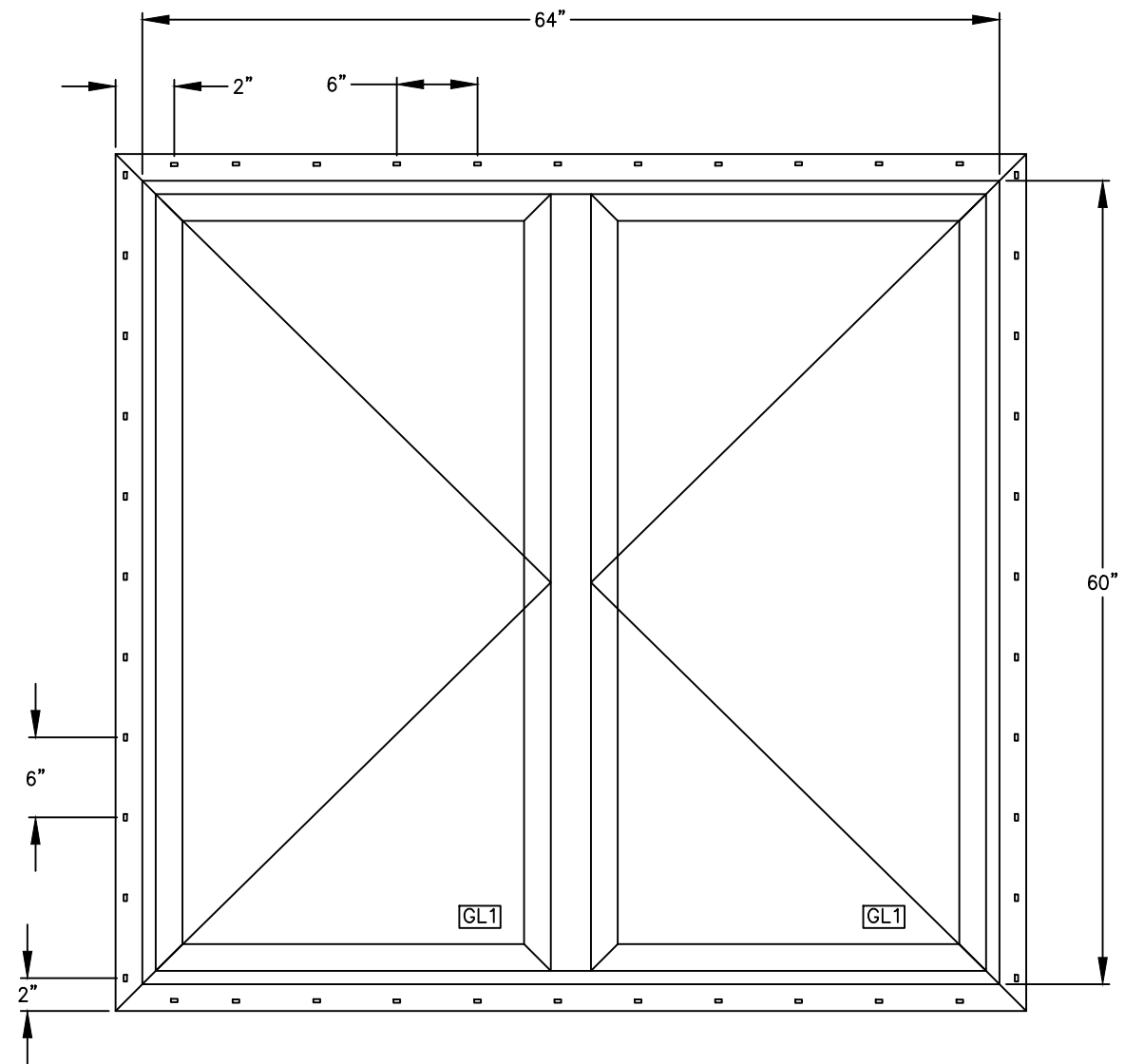
ASPECT/ENDURE T-MULL CASEMENT WINDOW (NON-IMPACT) MAXIMUM SIZE: 64" X 60" DESIGN PRESSURE: +50/-50 PSF NAIL FIN INSTALLATION METHOD
