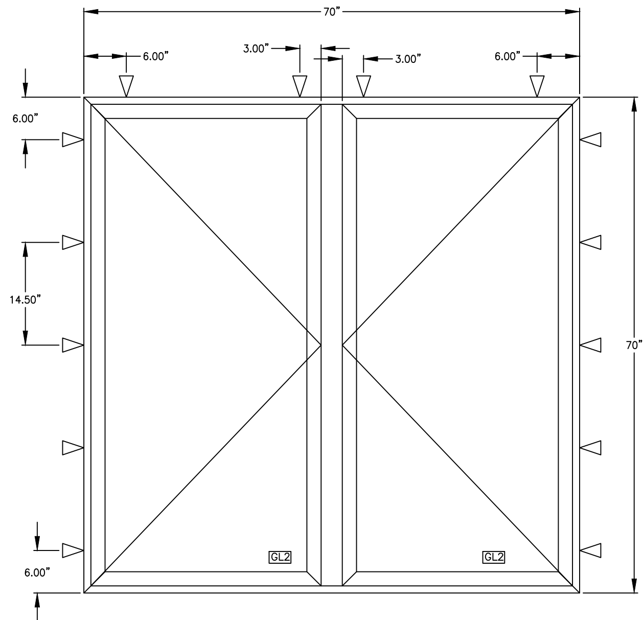
ASPECT/ENDURE T-MULL CASEMENT WINDOW (NON-IMPACT) MAXIMUM SIZE: 70" X 70" DESIGN PRESSURE: +45/-45 PSF THRU-FRAME INSTALLATION METHOD
