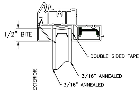
IG GLAZING GL2
