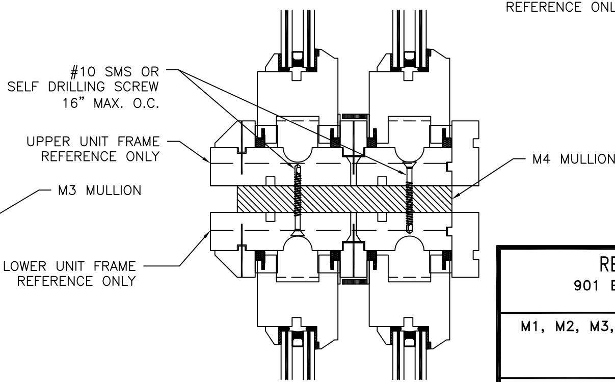
M4 MULLION TO WINDOW FRAME INSTALLATION DETAIL
