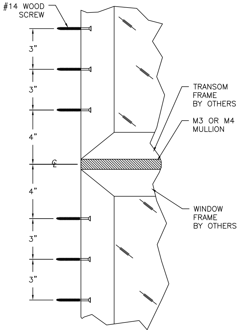
M3 OR M4 HORIZONTAL MULLION WOOD FRAMING OR 2X BUCK INSTALLATION
