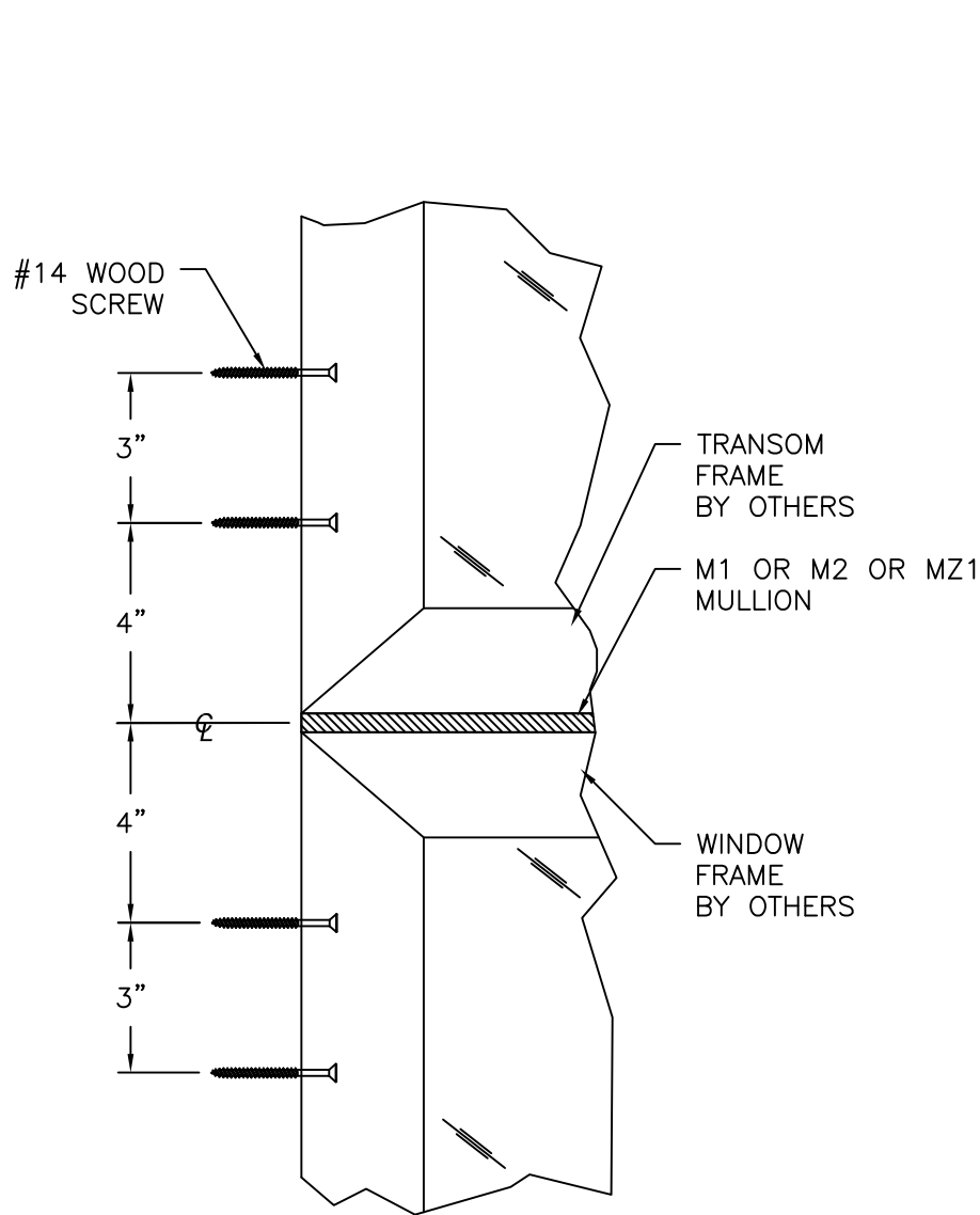
M1 OR M2 OR MZ1 HORIZONTAL MULLION WOOD FRAMING OR 2X BUCK INSTALLATION
