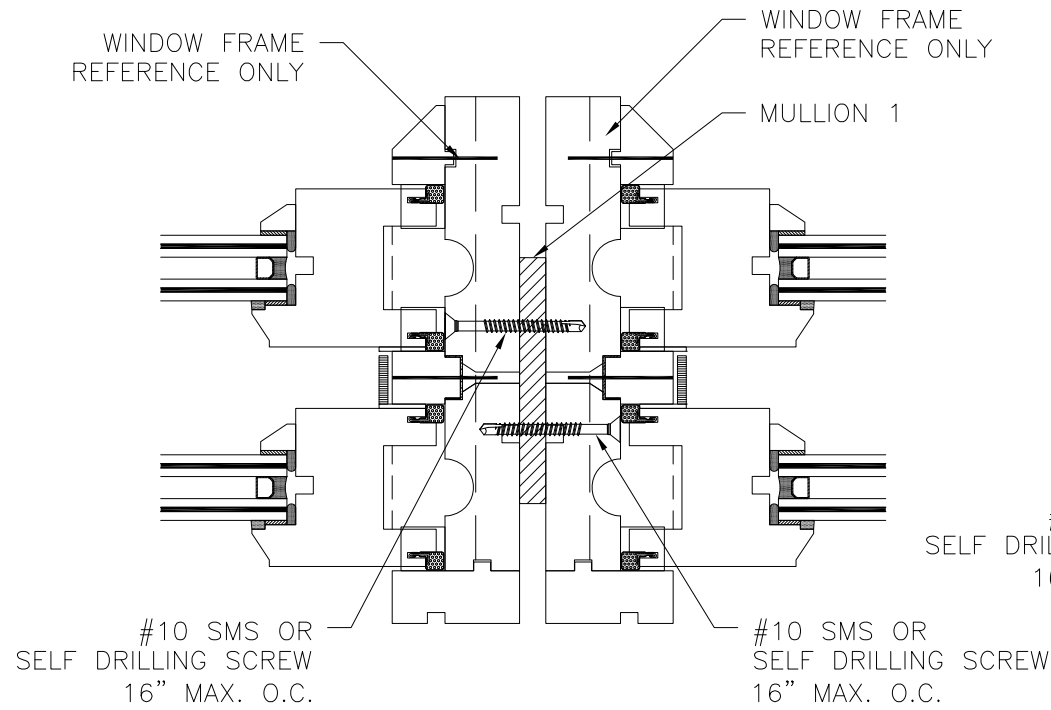
M1 MULLION TO WINDOW FRAME NSTALLATION DETAIL
