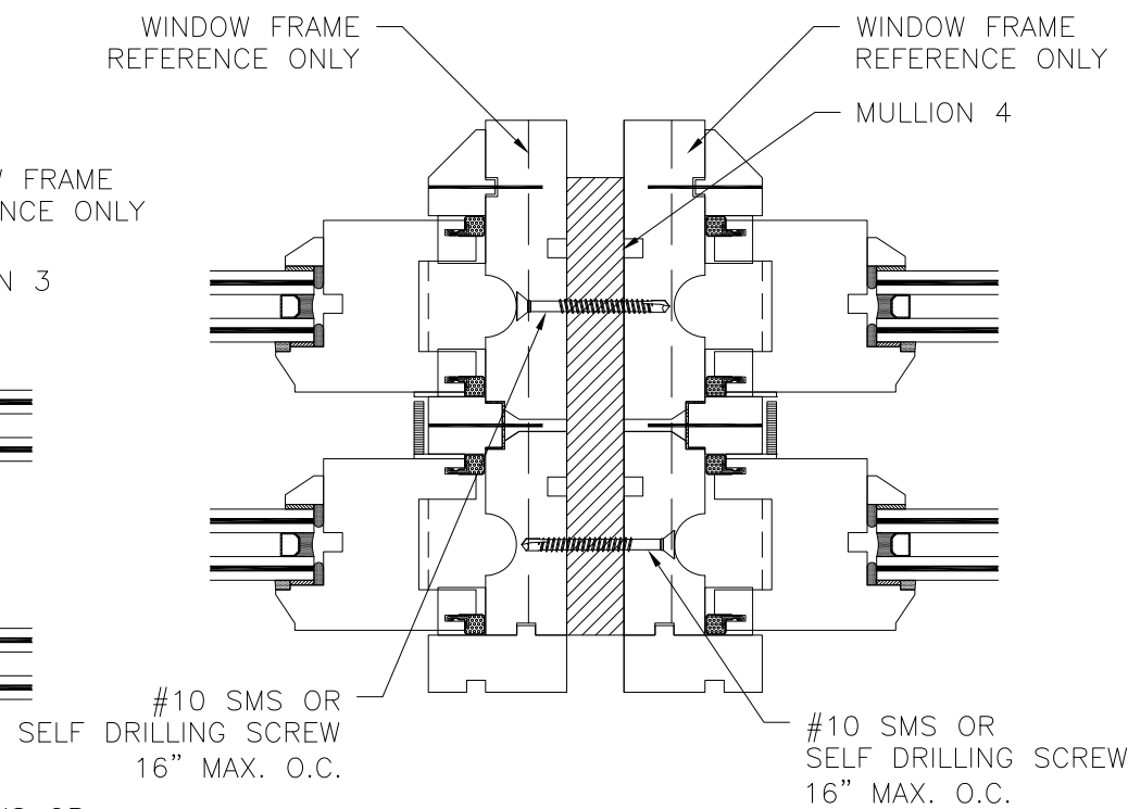
M4 MULLION TO WINDOW FRAME NSTALLATION DETAIL
