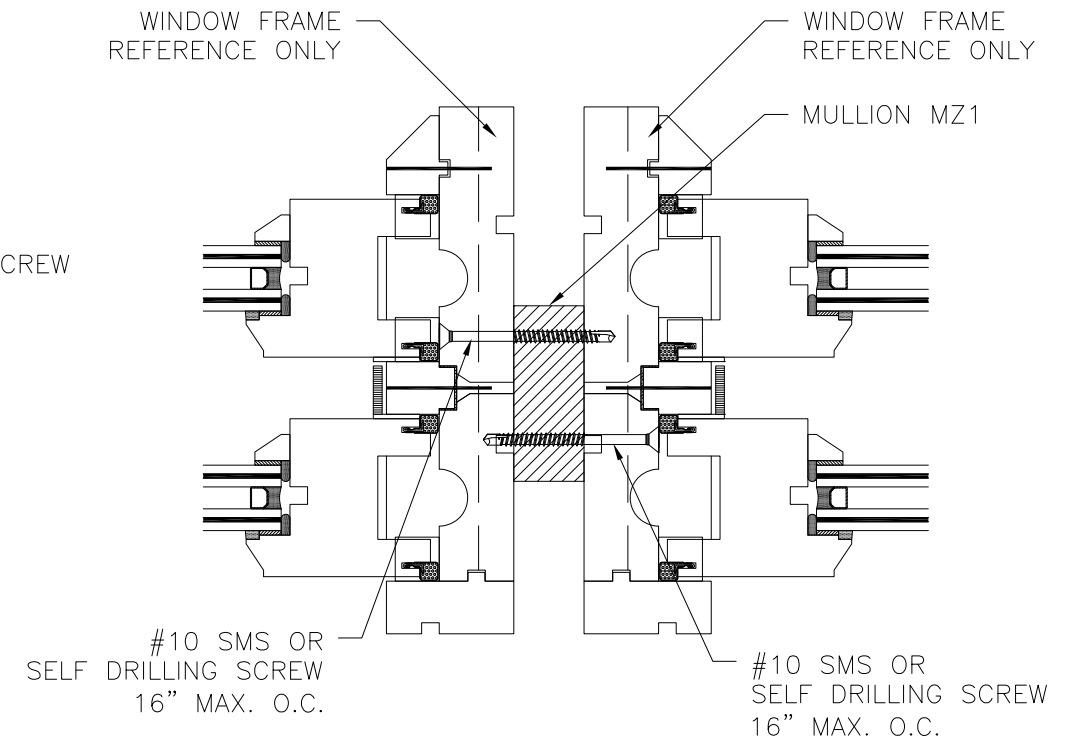
MZ1 MULLION TO WINDOW FRAME NSTALLATION DETAIL
