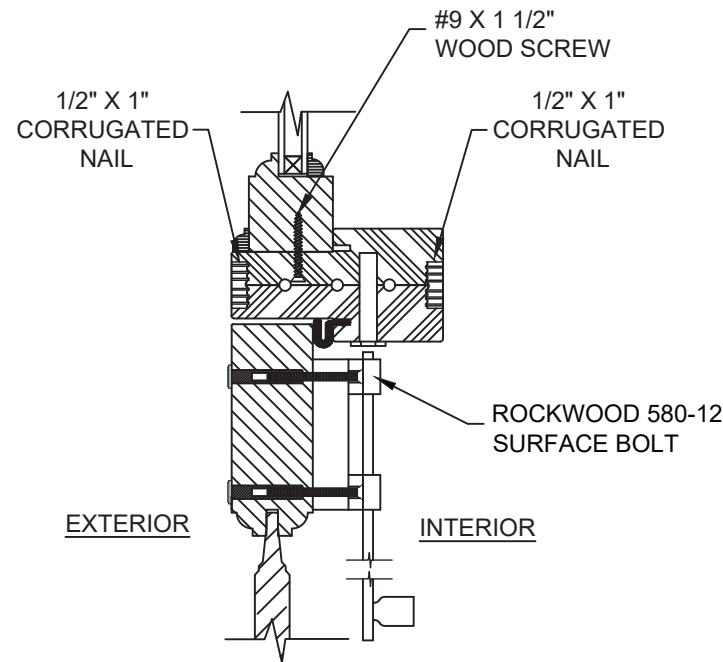
VERTICAL SECTION DOUBLE JAMB HORIZONTAL MULL AT DOOR PANEL
