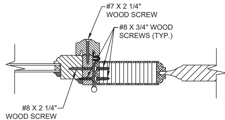
HORIZONTAL SECTION HINGE STILE AT VERTICAL MULL
