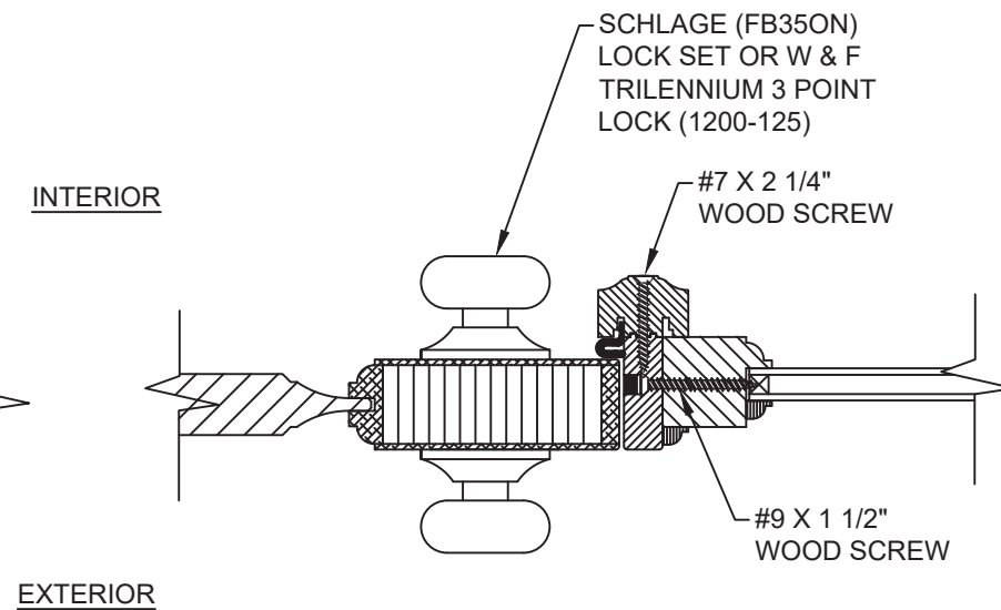
HORIZONTAL SECTION LOCK STILE AT VERTICAL MULL
