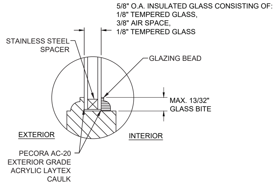
GLAZING DETAIL
