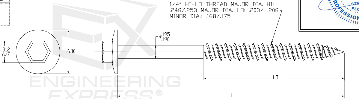
1/4" SOLID SET™ LG HEX WASHER HEAD SCREW (CS AND 410 SS)
