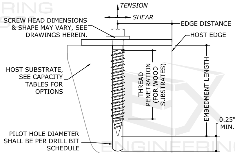
1 TYPICAL SECTION 2 NTS SECTION VIEW
