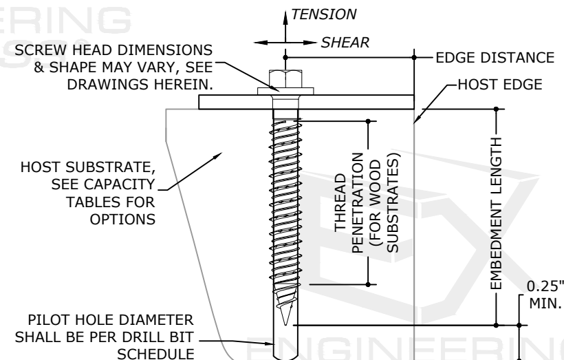
1 TYPICAL SECTION 4 NTS SECTION VIEW
