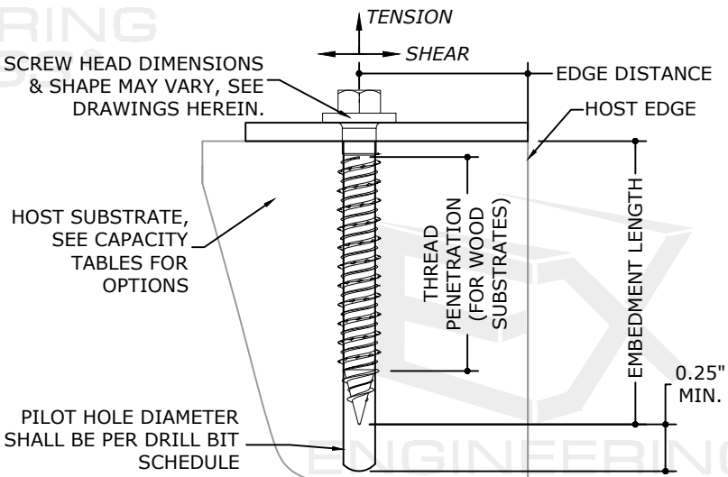
1 TYPICAL SECTION 3 NTS SECTION VIEW
