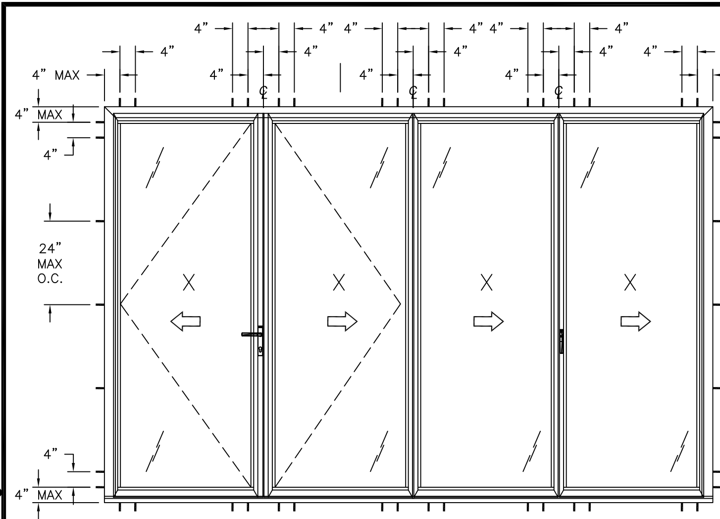
ANCHORING LAYOUT FOR SYSTEMS RATED HIGHER THAN 40PSF
