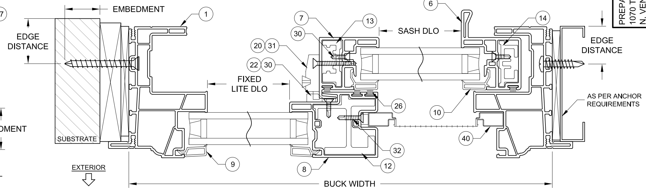
3 JAMB FLANGE FRAME X-SECTION THRU 1X INTO 2X WOOD OR MASONRY
