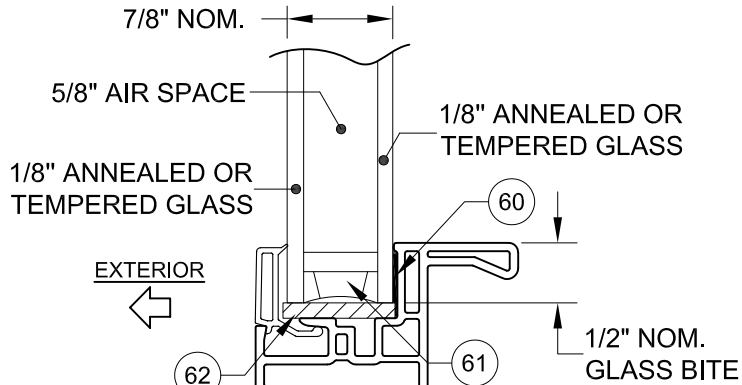
GLASS TYPE 1
