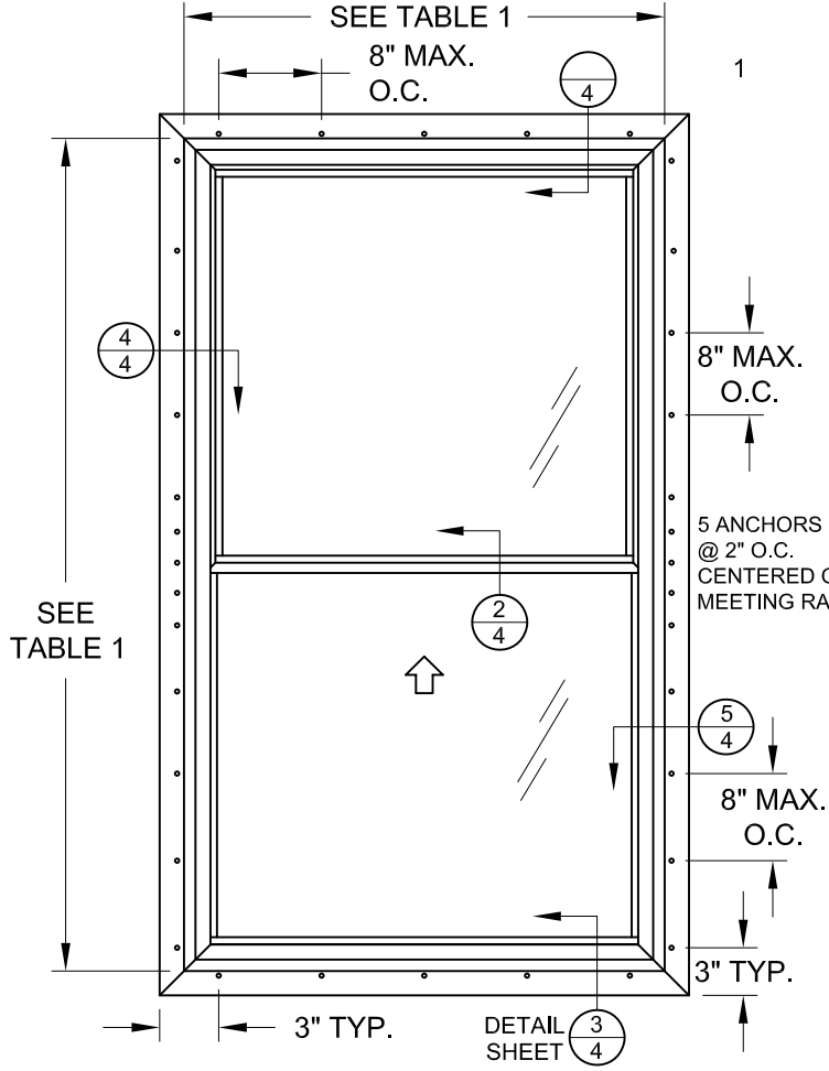
TYP. FIN ANCHOR LOCATIONS (A) (INTEGRAL FIN FRAME, EQUAL-LITE SHOWN, ORIEL SIMILAR)
