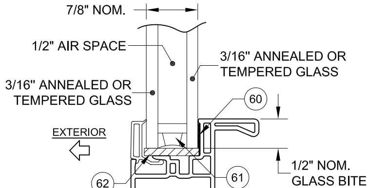
GLASS TYPE 2
