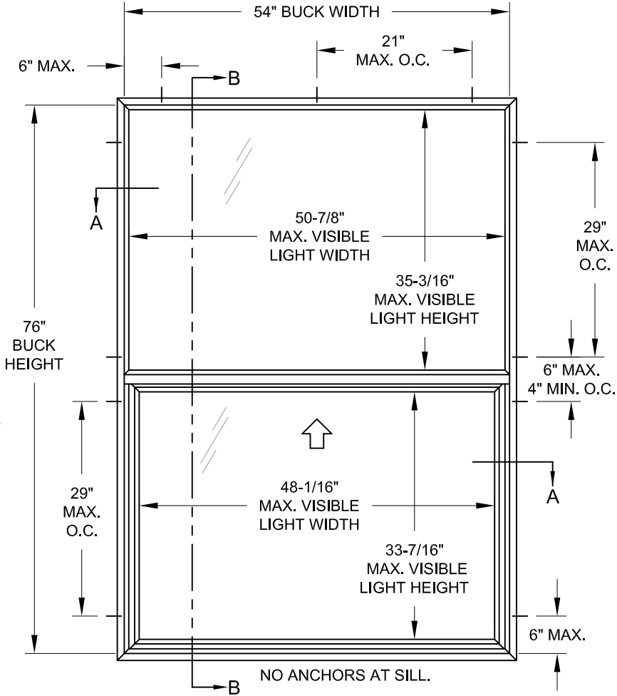
TYP. ANCHOR LOCATIONS @ TESTED SIZE (FLANGE / EQUAL LEG FRAME)
