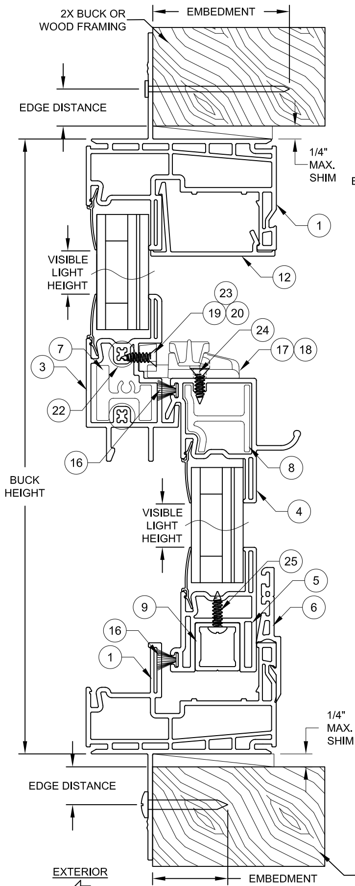
VERTICAL SECTION D-D
