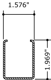
13 REINFORCEMENT 268742
