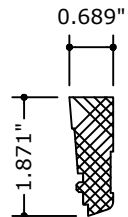
11 DISTANCE PIECE 241043
