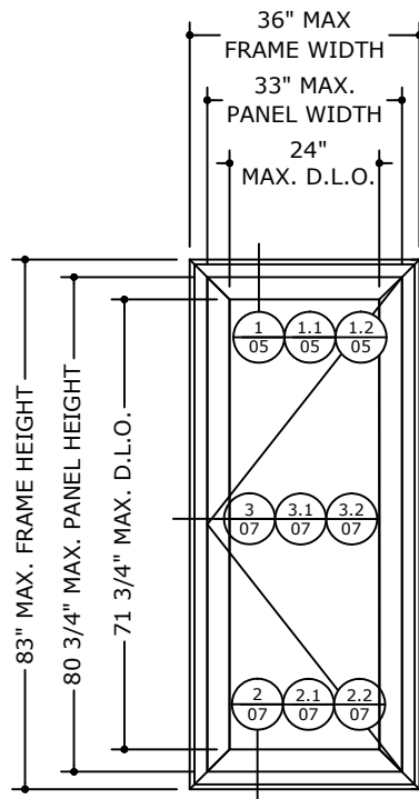
TYPICAL SINGLE (X) DOOR ELEVATION
