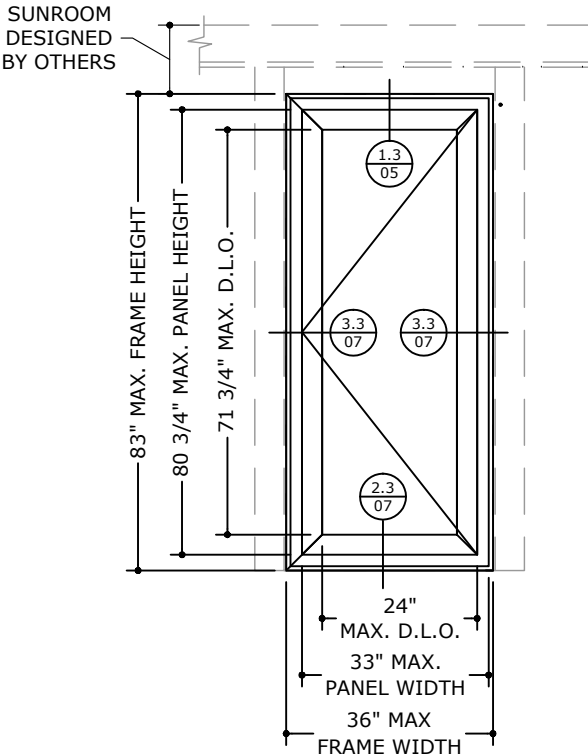
SUNROOM ELEVATION
