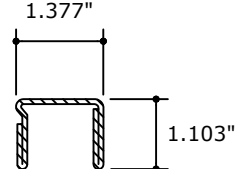
5 REINFORCEMENT 244536
