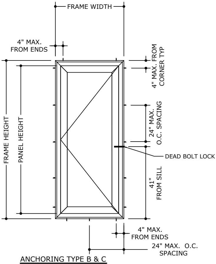
TYPICAL ANCHOR SPACING LAYOUT
