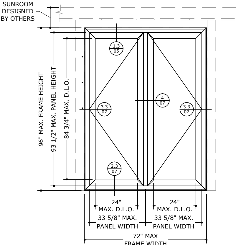
SUNROOM ELEVATION
