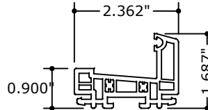
4 VINYL SILL 601235
