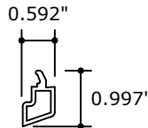
7 GLAZING STOP 560600
