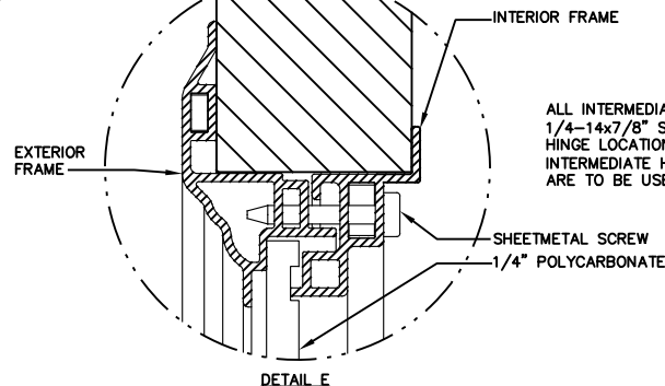
DETAIL E
