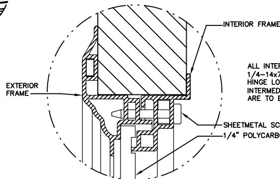
DETAIL E
