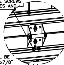
DETAIL H
