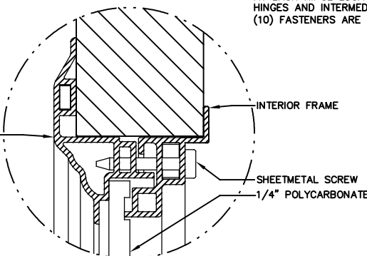
DETAIL D
