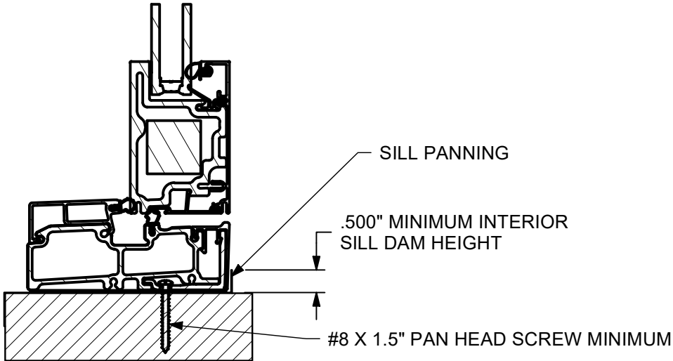
PERFORMANCE SILL (SHOWN) (LOW PROFILE SILL INSTALLATION SAME)
