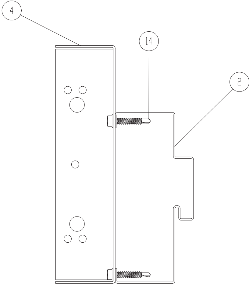
FRAME JAMB (ITEM NO. 2) TO SUBFRAME (ITEM 4) FASTENING
