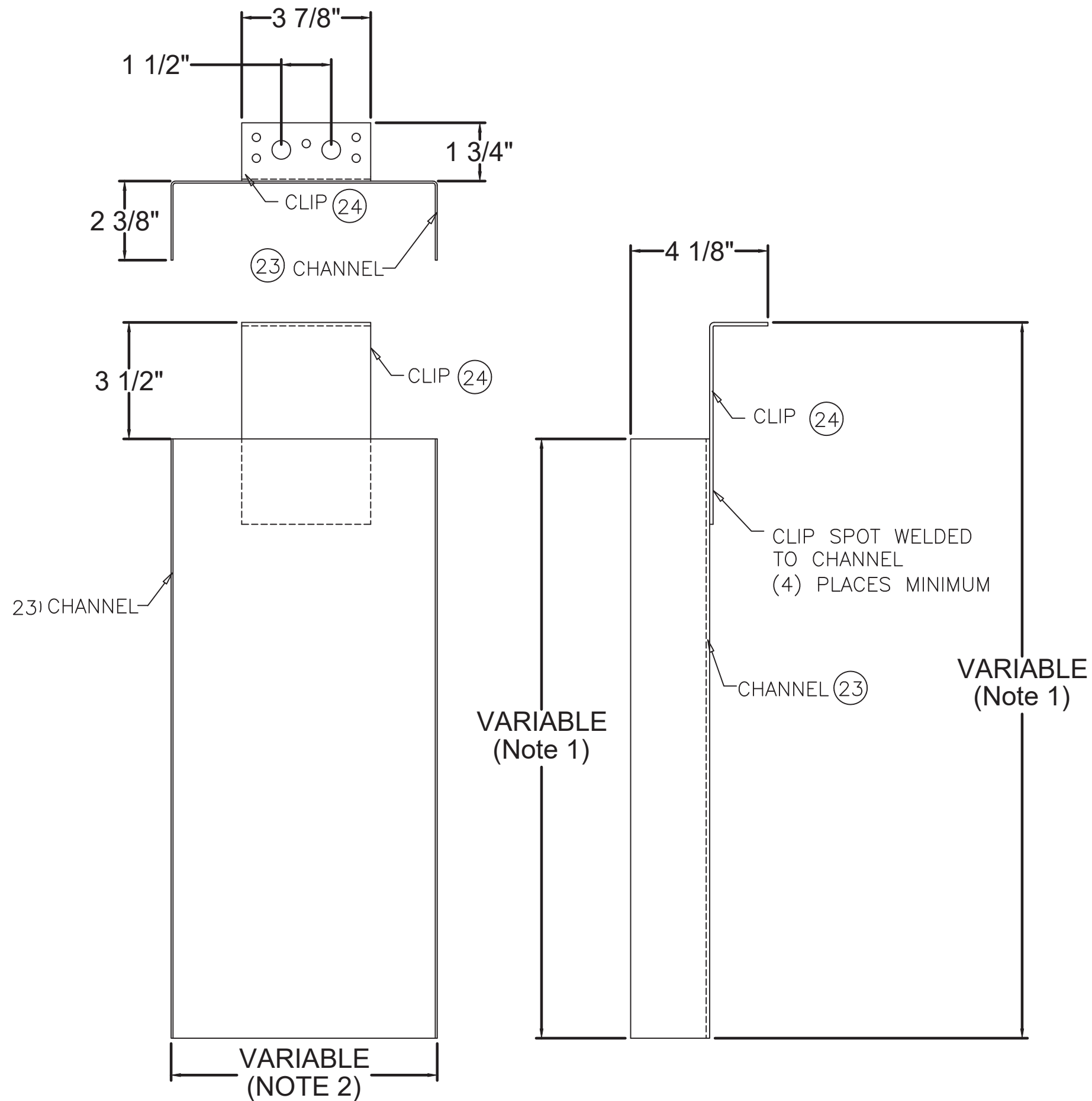
(22) JAMB EXTENSION ASSEMBLY
