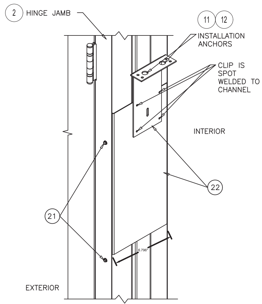
JAMB EXTENSION ASSEMBLY DETAIL
