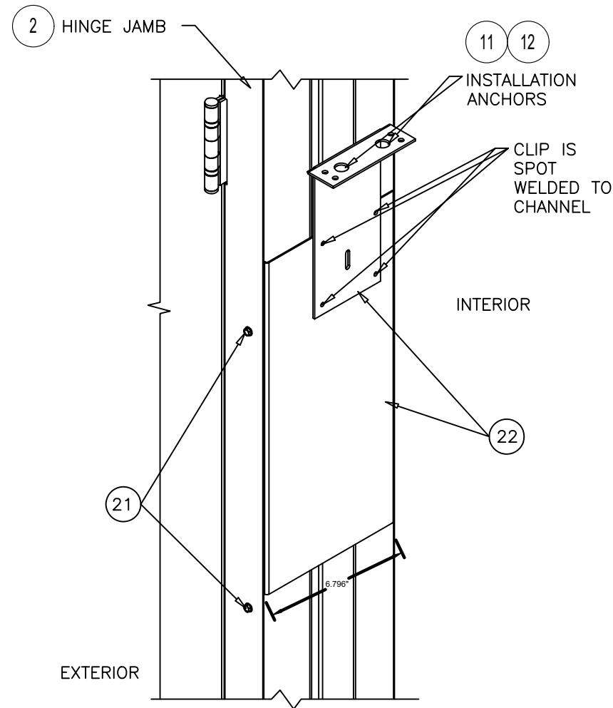
JAMB EXTENSION ASSEMBLY DETAIL
