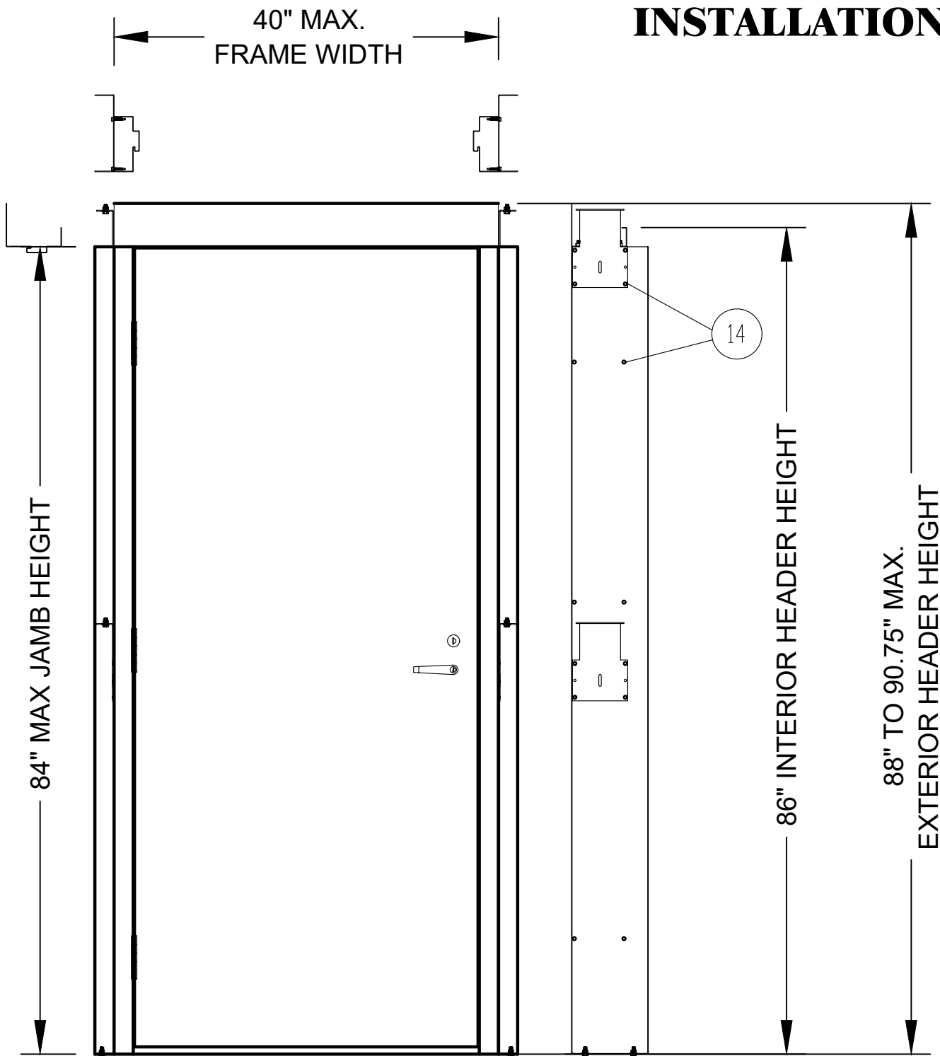
ELEVATION EXTERIOR
