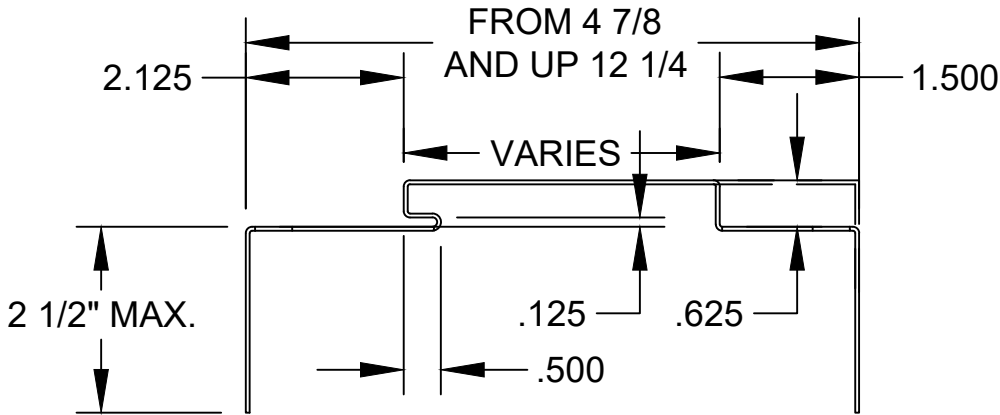
1 HOLLOW METAL FRAME HEAD
