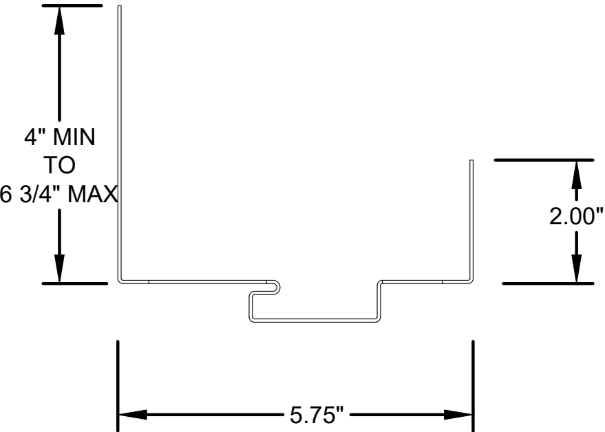
1 HOLLOW METAL FRAME HEAD (STANDARD)
