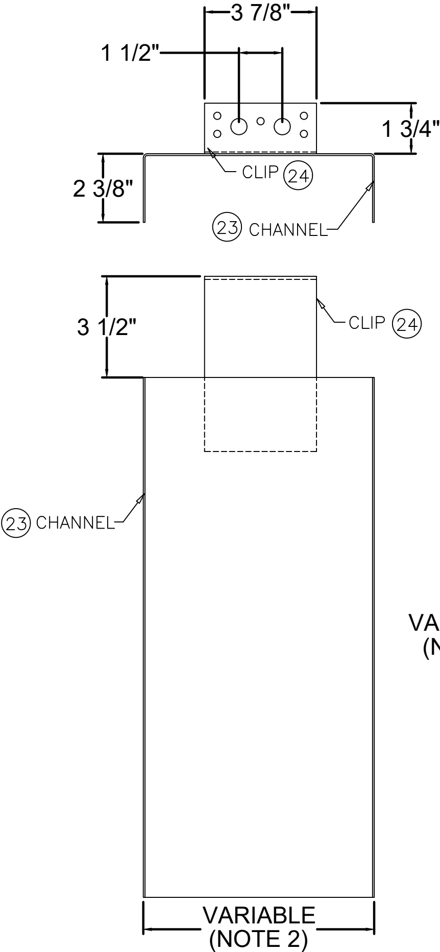
(22) JAMB EXTENSION ASSEMBLY
