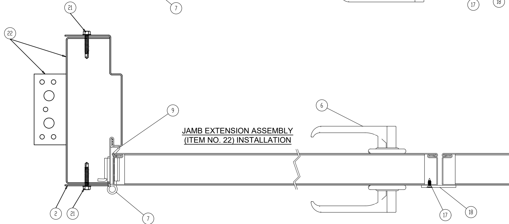
HORIZONTAL CROSS SECTION INSTALLATIONS
