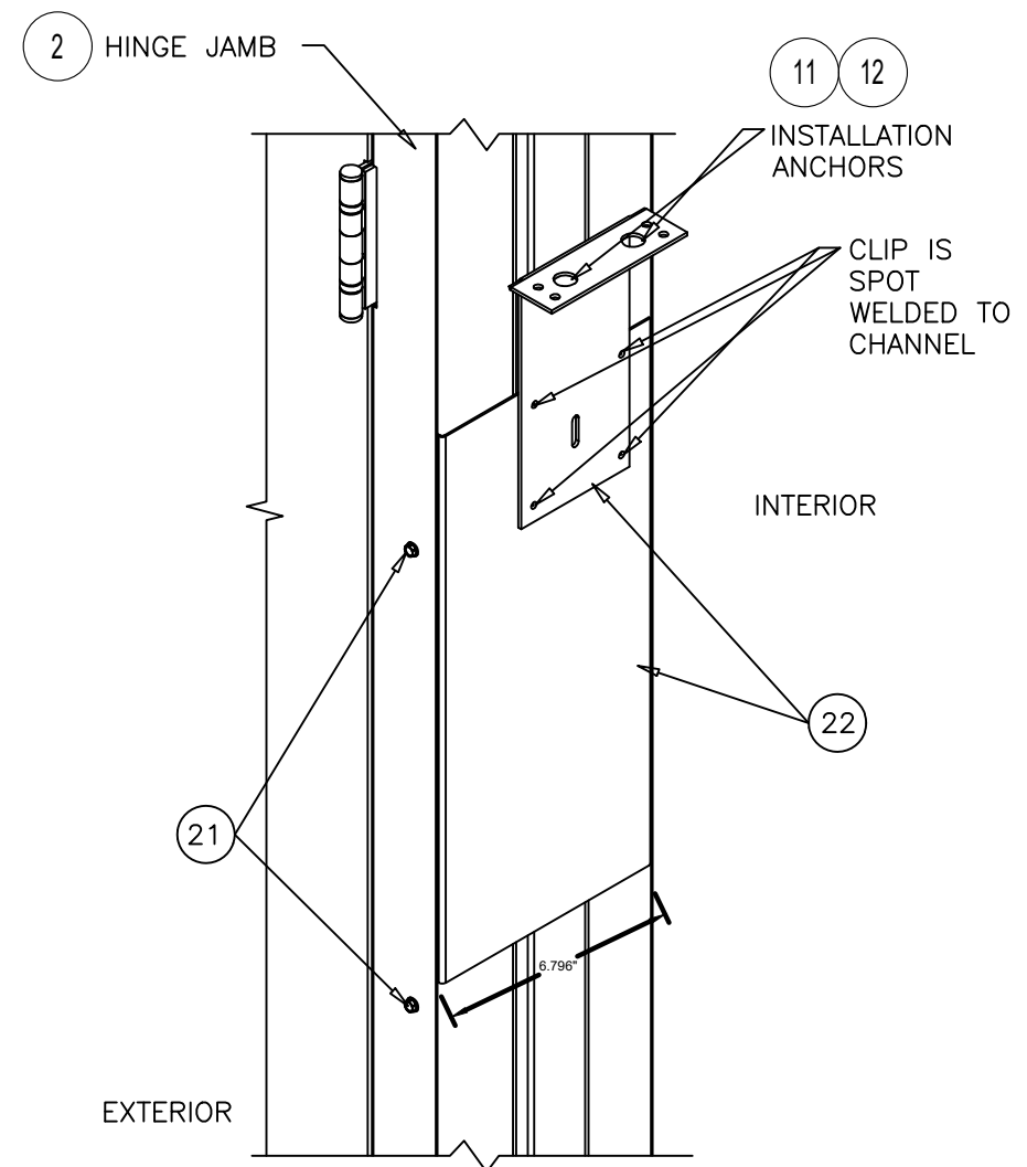
JAMB EXTENSION ASSEMBLY DETAIL
