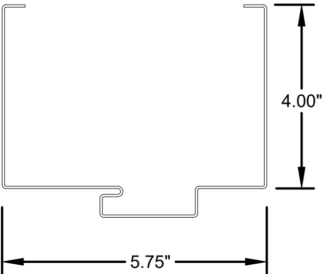
20 HOLLOW METAL FRAME HEAD (STANDARD)
