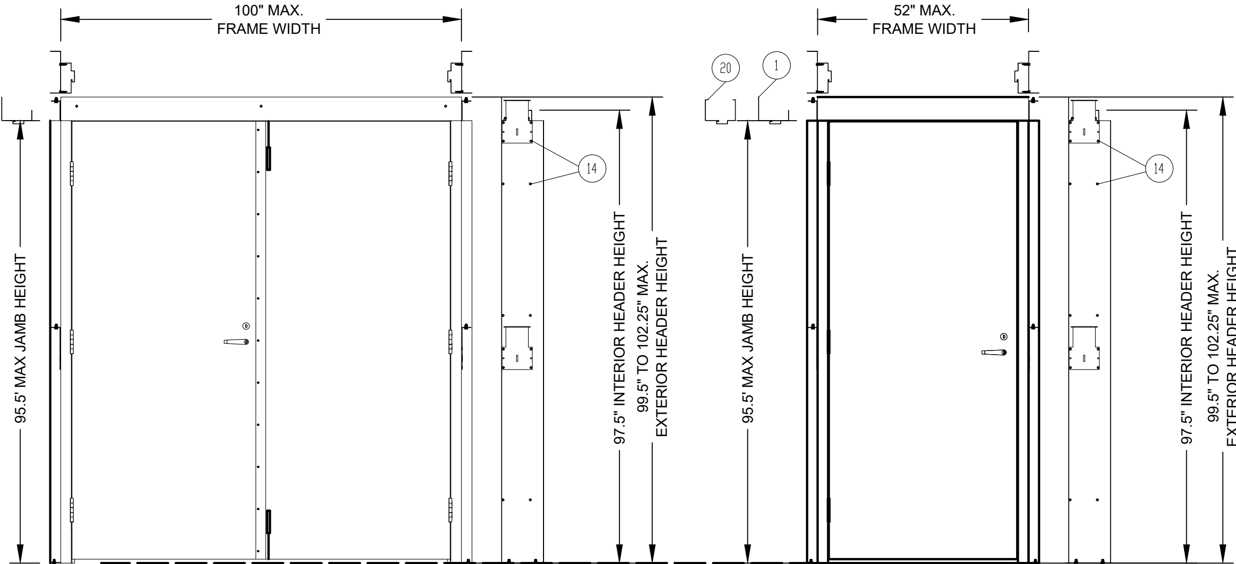
ELEVATION EXTERIOR CYLINDRICAL LOCK & DEADBOLT SHOWN. MORTISE LOCK AND PANIC BAR EXIT DEVICE ALSO APPROVED.
