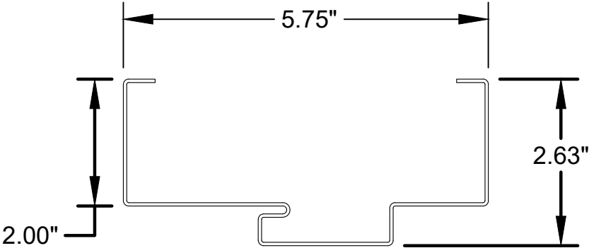
2 HOLLOW METAL FRAME JAMB (STANDARD)
