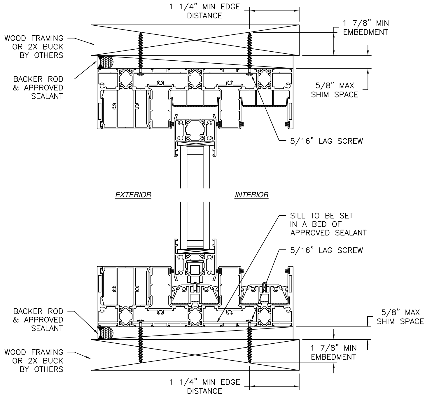
VERTICAL CROSS SECTION STANDARD SILL SHOWN, OTHER SILLS SIMILAR WOOD FRAMING OR 2X BUCK INSTALLATION
