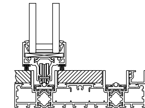
2-TRACK UNIT WITH MINIMAL SILL
