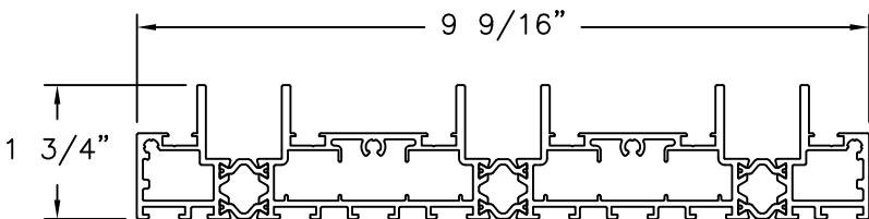
3-TRACK MINIMAL SILL
