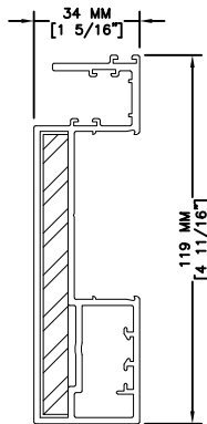
Part No. 5-210-33-X Item Description: 6063-T5 ALUMINUM LATERAL PANEL CONNECTION PROFILE, OPPOSITE DIRECTION (STILE) WITH STEEL REINFORCEMENT
