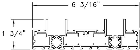
2-TRACK MINIMAL SILL
