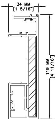
Part No. 5-210-31-X Item Description: 6063-T5 ALUMINUM LATERAL PANEL CONNECTION PROFILE, PARALLEL DIRECTION (STILE) WITH STEEL REINFORCEMENT
