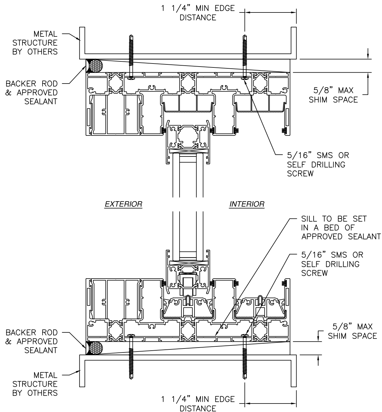
VERTICAL CROSS SECTION STANDARD SILL SHOWN, OTHER SILLS SIMILAR METAL STRUCTURE INSTALLATION
