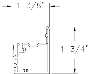
LOCK RAIL (8896) EXTRUDED VINYL PVC
