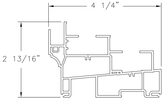
JAMB FRAME (10008690) EXTRUDED VINYL PVC
