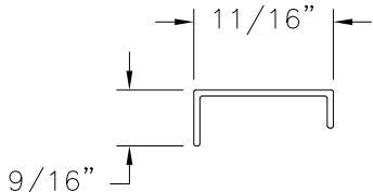
REINFORCEMENT (10300096) ALUMINUM 6005-T5, 6061-T6 OR 6105-T5
