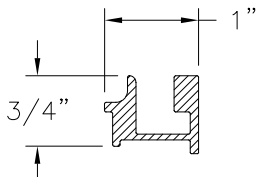
REINFORCEMENT (10300083) ALUMINUM 6005-T5, 6061-T6 OR 6105-T5
