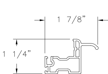
TOP LIFT RAIL (8894) EXTRUDED VINYL PVC
