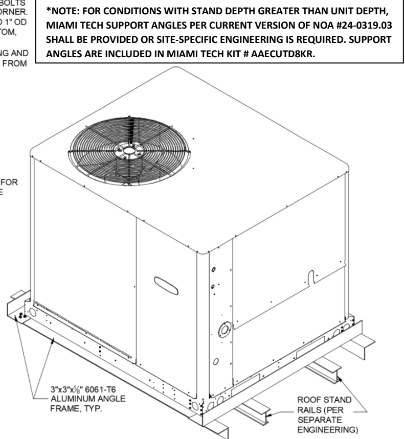
7 UNIT MOUNT ON ROOF STAND AND FRAME SCALE: NTS ISOMETRIC VIEW
