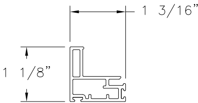
SASH STILE/BOTTOM RAIL (V-705) EXTRUDED RIGID PVC
