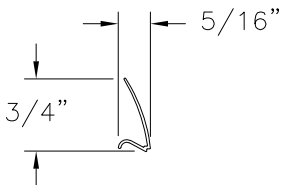
GLAZING BEAD (1718R) EXTRUDED RIGID PVC
