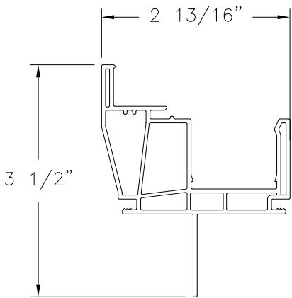
HEAD FRAME (V-772) FIN INSTALLATION EXTRUDED RIGID PVC
