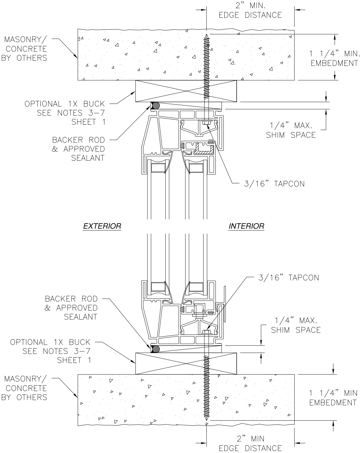
VERTICAL CROSS SECTION MASONRY/CONCRETE INSTALLATION
