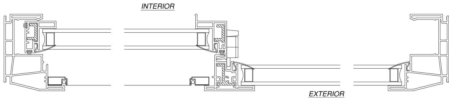
HORIZONTAL CROSS SECTION FINLESS FRAME
