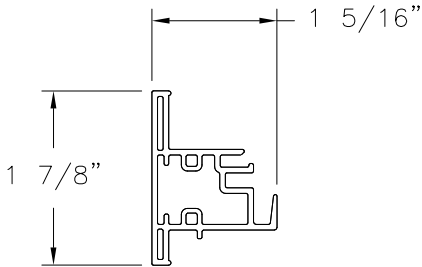
MEETING RAIL (V-706) EXTRUDED RIGID PVC
