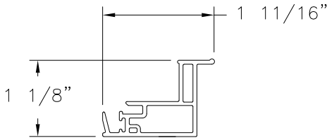
SASH LOCK RAIL (V-704) EXTRUDED RIGID PVC
