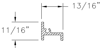
REINFORCEMENT (2230-C) ALUMINUM 6063-T5
