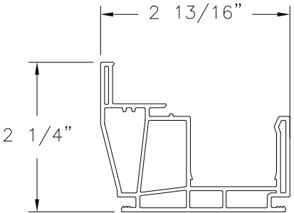
HEAD FRAME (V-772) EXTRUDED RIGID PVC
