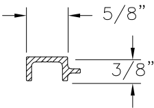
REINFORCEMENT (2243-A) ALUMINUM 6063-T5
