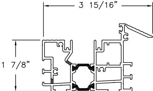
INTERMEDIATE SILL ALUMINUM 6063-T5
