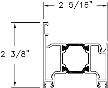
STILE/ RAIL ALUMINUM 6063-T5
