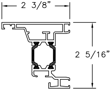
RUNNING POST ALUMINUM 6063-T5
