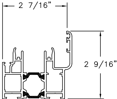
RAISED SILL ALUMINUM 6063-T5
