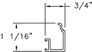
GLAZING BEAD ALUMINUM 6063-T5
