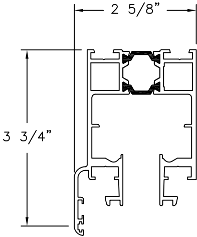
EXTENDED OR TOP HUNG HEAD ALUMINUM 6063-T5
