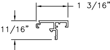
EXTENDER ALUMINUM 6063-T5
