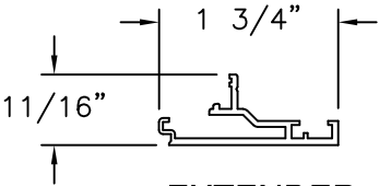
EXTENDER ALUMINUM 6063-T5
