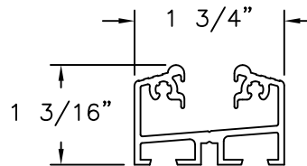
STANDARD SILL ALUMINUM 6063-T5
