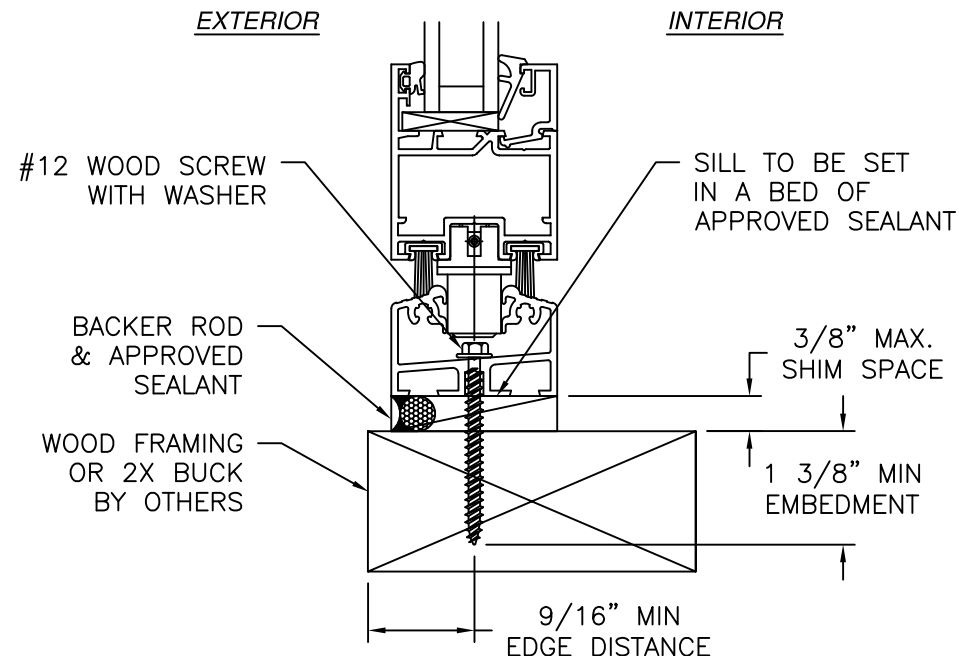
VERTICAL CROSS SECTION WOOD FRAMING OR 2X BUCK INSTALLATION STANDARD SILL SHOWN, OTHER SILLS SIMILAR
