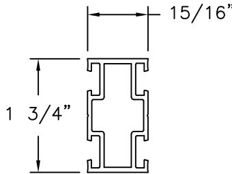
FRAME STILE ALUMINUM 6063-T5
