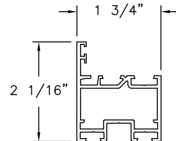
PANEL FRAME ALUMINUM 6063-T5
