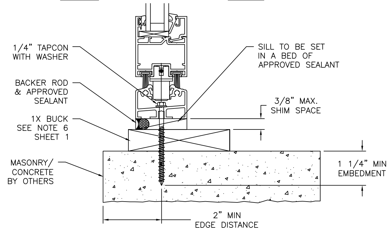
VERTICAL CROSS SECTION CONCRETE/MASONRY WITH 1X BUCK INSTALLATION FOR CONCRETE/MASONRY WITHOUT 1X BUCK REFER TO JAMB INSTALLATION DETAIL STANDARD SILL SHOWN, OTHER SILLS SIMILAR
