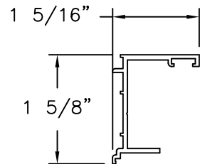
FRAME EXTENDER ALUMINUM 6063-T5
