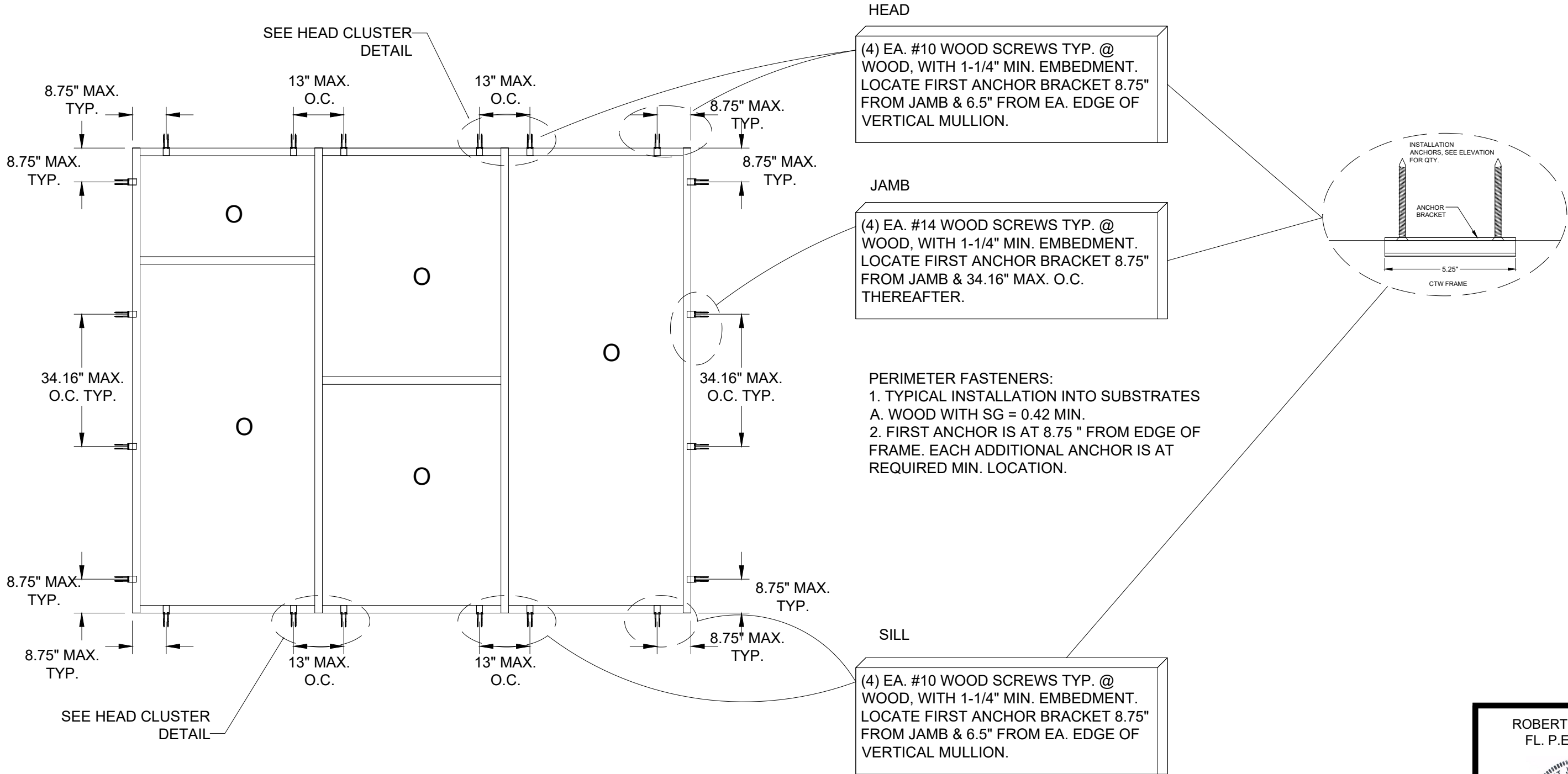
SERIES 50 F CAPPED ALUMINUM CURTAIN WALL WOOD FRAME INSTALLATION (SEE SHEET 4 FOR CONCRETE/CMU INSTALLATION) EXTERIOR VIEW
