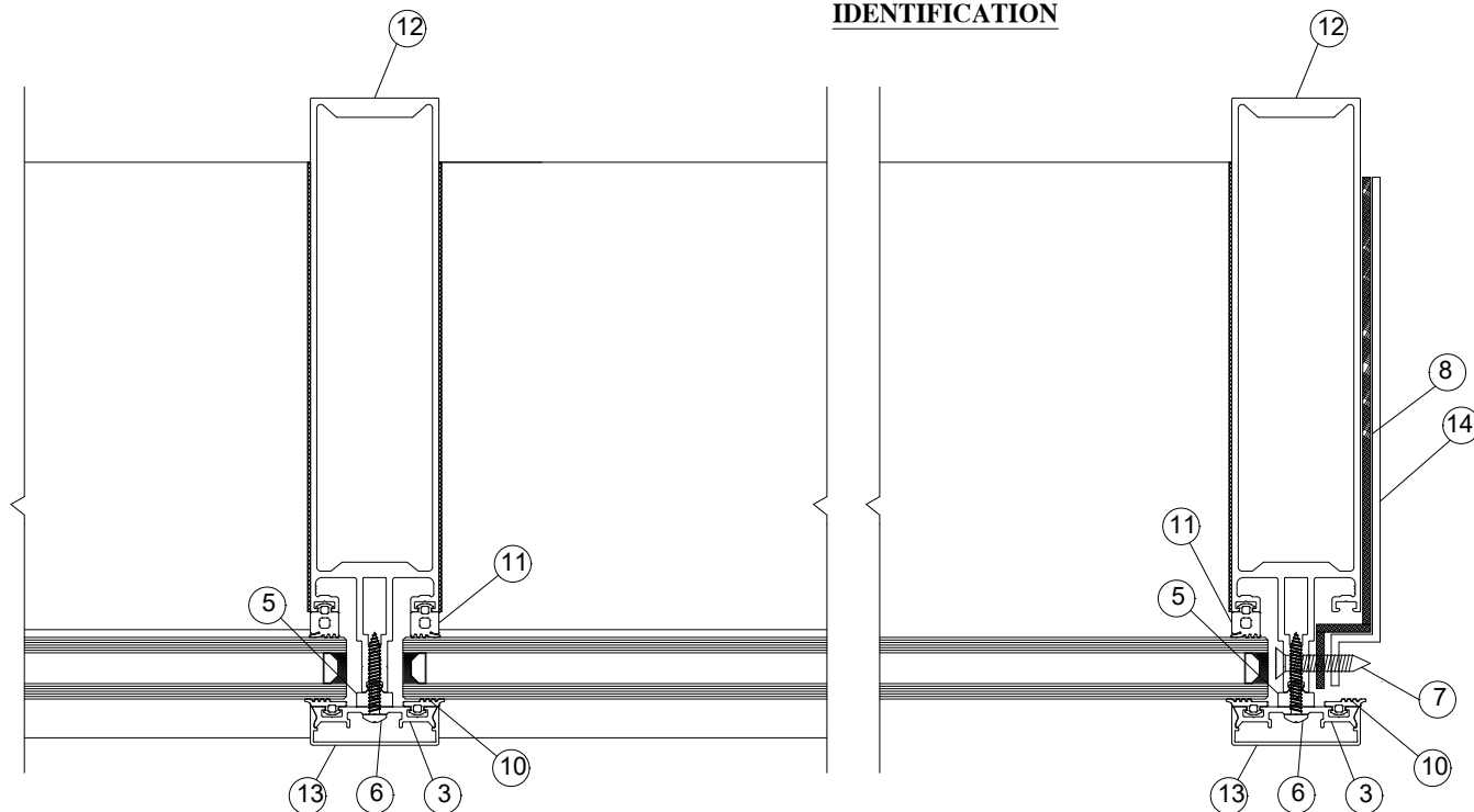
TYPICAL CROSS SECTION FOR PARTS IDENTIFICATION
