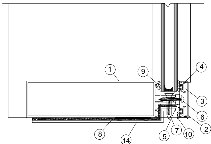
TYPICAL CROSS SECTION FOR PARTS IDENTIFICATION
