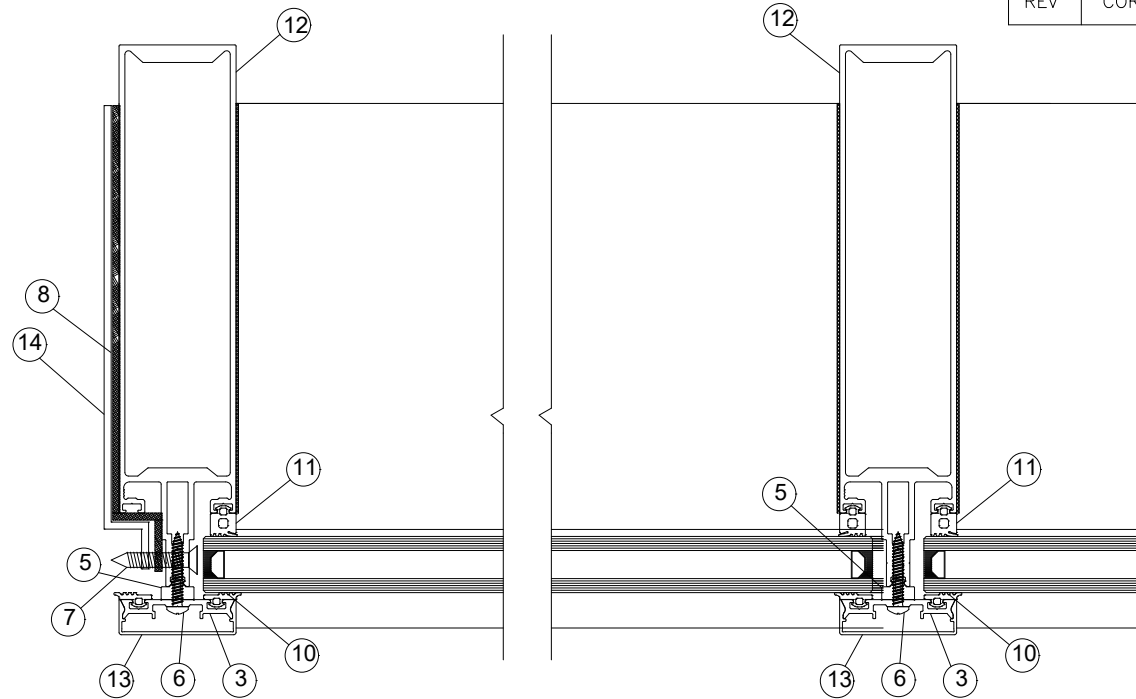
TYPICAL CROSS SECTION FOR PARTS IDENTIFICATION
