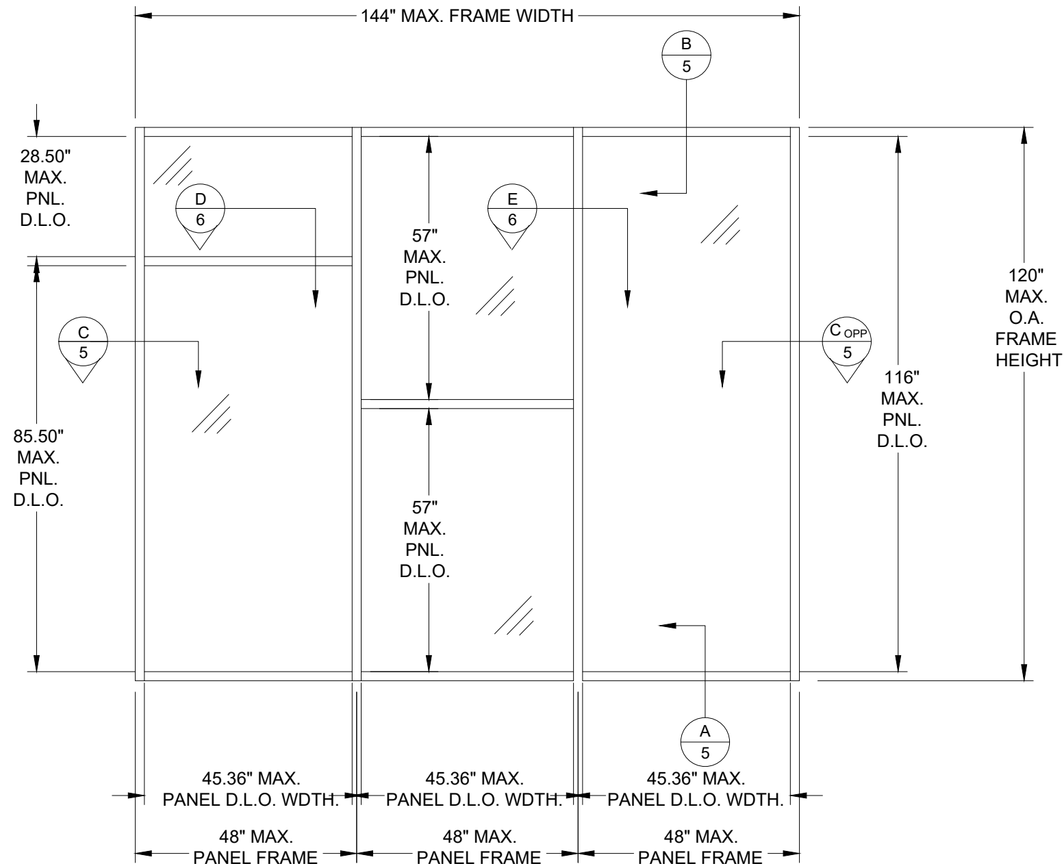
SERIES 50 F CAPPED ALUMINUM CURTAIN WALL WITH NON-REINFORCED MULL EXTERIOR VIEW
