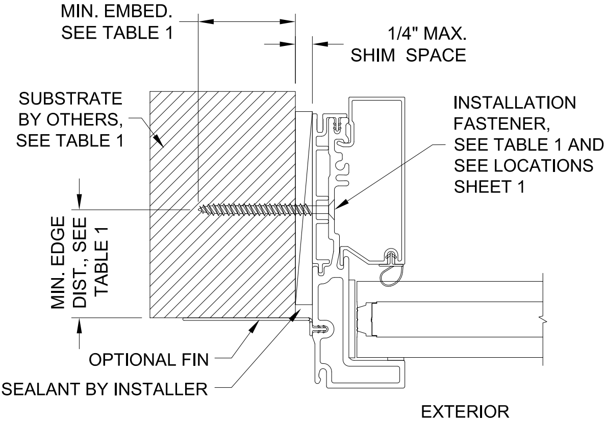
TYPICAL SECTION INSTALLATION
