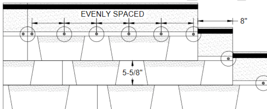
Figure 1: Six (6) Nail Pattern (minimum)
