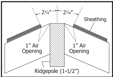
Ridgepole Diagram
