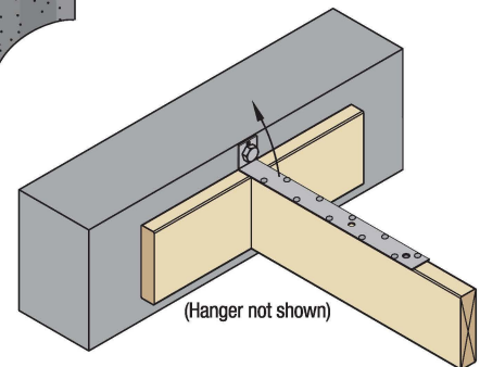
LTT20B as Tension Tie
