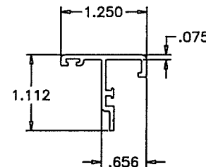
CGI-505 ASTRAGAL
