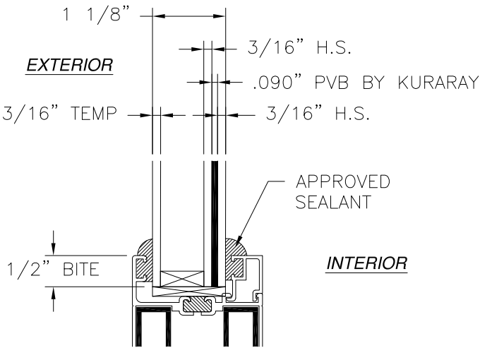
GLAZING DETAIL GL1
