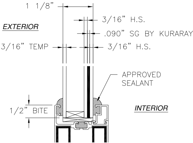
GLAZING DETAIL GL2
