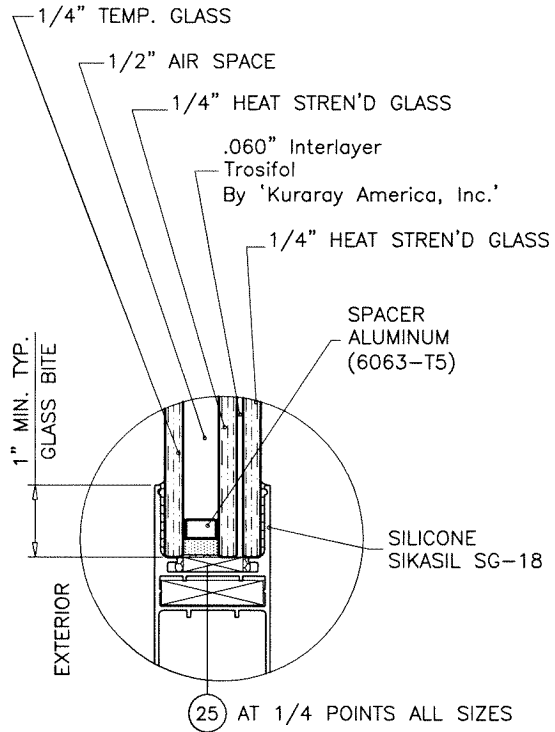
GLASS TYPE 'A1' 1-5/16" OVERALL INSUL. LAM. GLASS
