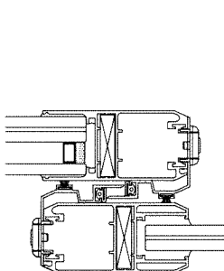
STD. INTERLOCKS
