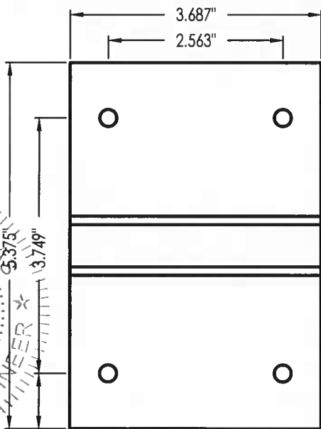
12 MULLION ANCHOR (SUN-262)
