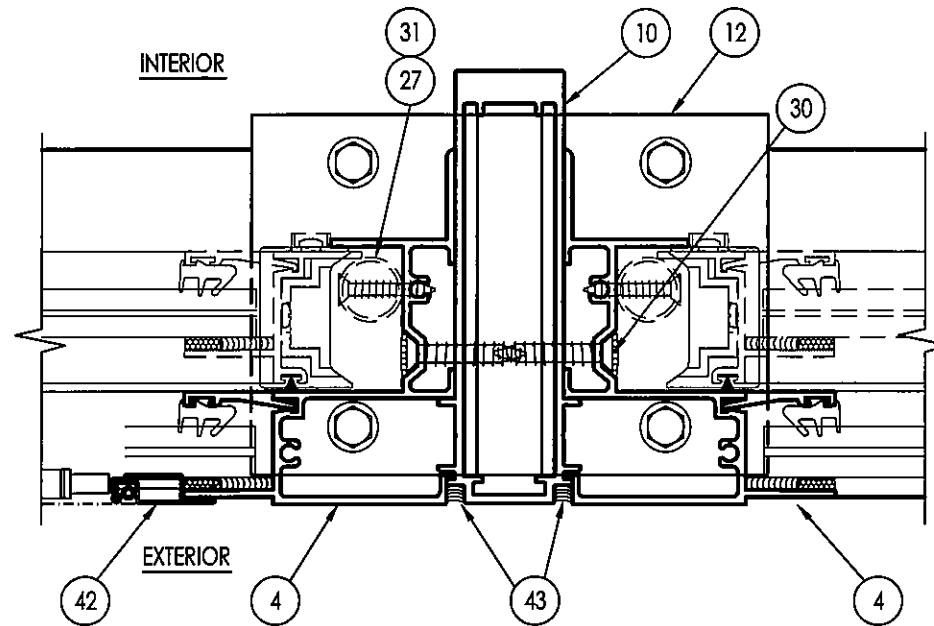
E MULLION 2
