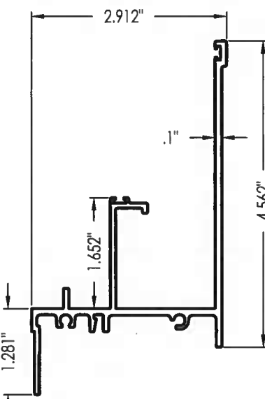
11 INTERMEDIATE FRAME SILL (SUN-259)
