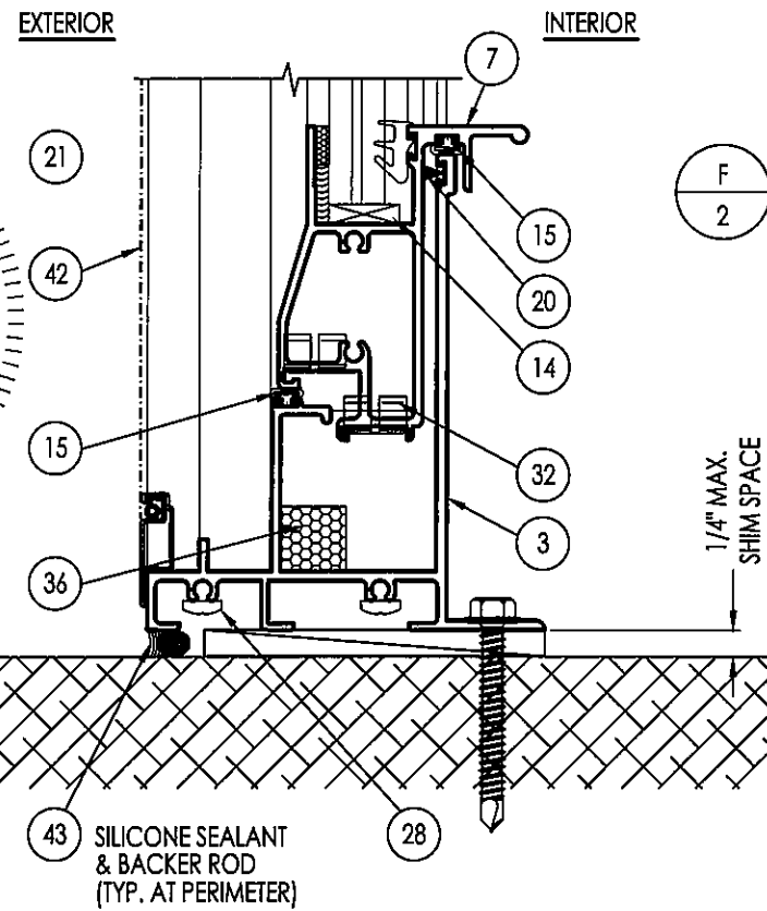
C FRAME SILL 2
