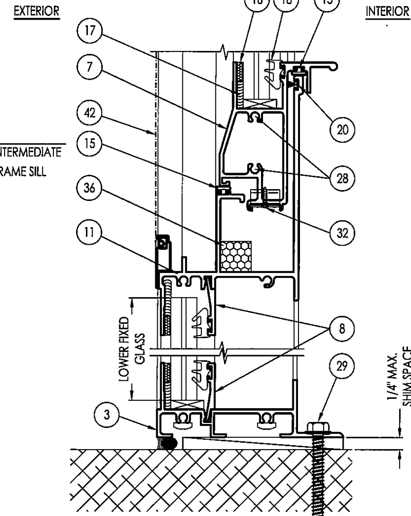
G FIXED WINDOW SILL 2
