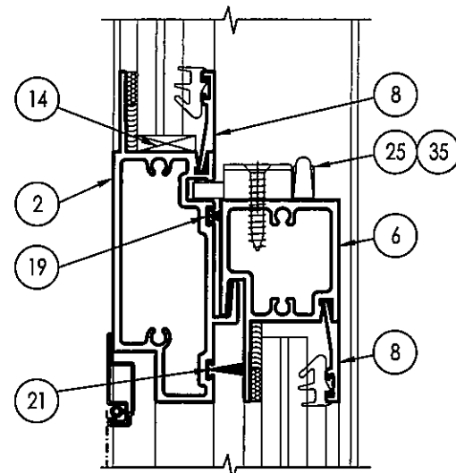
B MEETING RAILS 2
