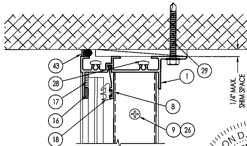
A FRAME HEAD 2
