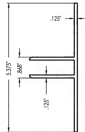
12 MULLION ANCHOR (SUN-262)
