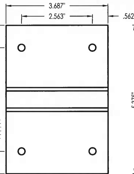
12 MULLION ANCHOR (SUN-262)
