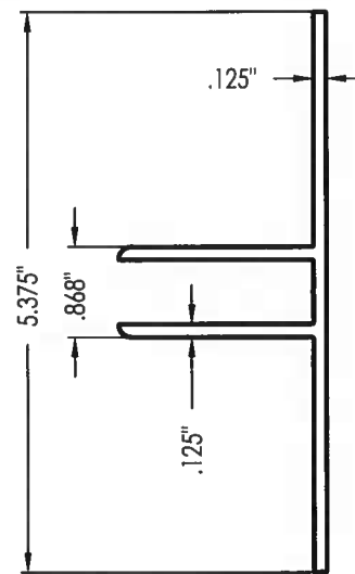
12 MULLION ANCHOR (SUN-262)
