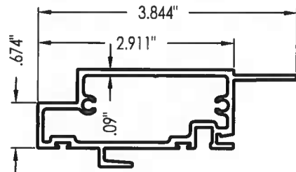
2 FIXED MEETING RAIL (SUN-252)
