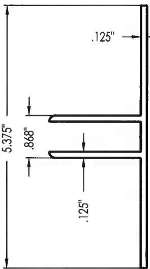
12 MULLION ANCHOR (SUN-262)
