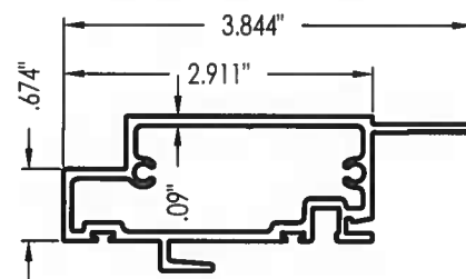
2 FIXED MEETING RAIL (SUN-252)
