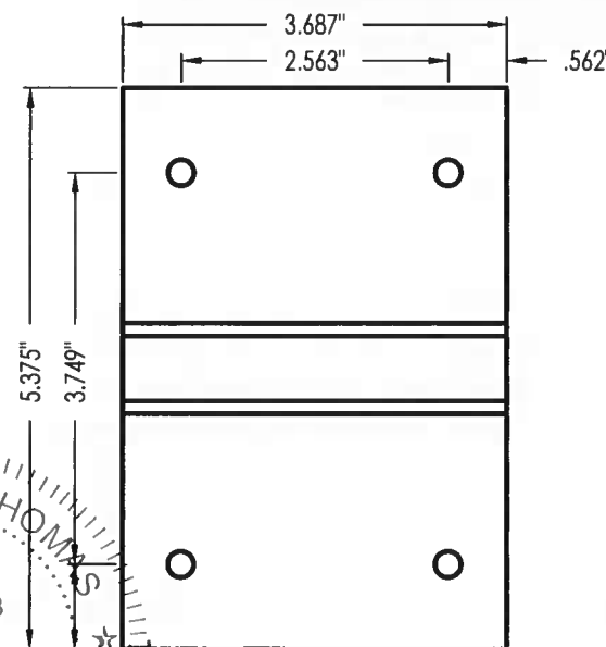
12 MULLION ANCHOR (SUN-262)
