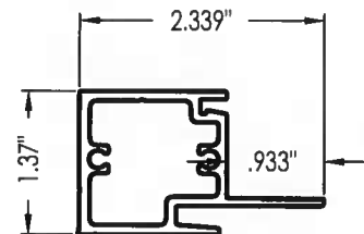
6 SASH TOP RAIL (SUN-256)
