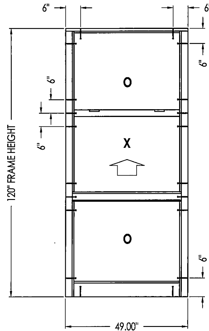
APPROVED ANCHORS 5/16" ITW TAPCONS
