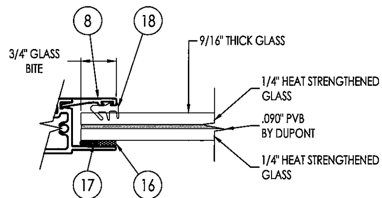
G4 GLAZING DETAIL
